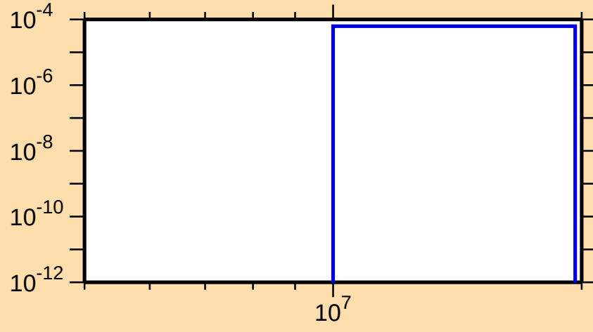
\sigma vs. E for ^{185}\text{W}(n,np)
