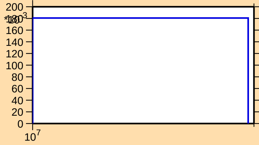
\sigma vs. E for ^{185}\text{W}(n,3n)
