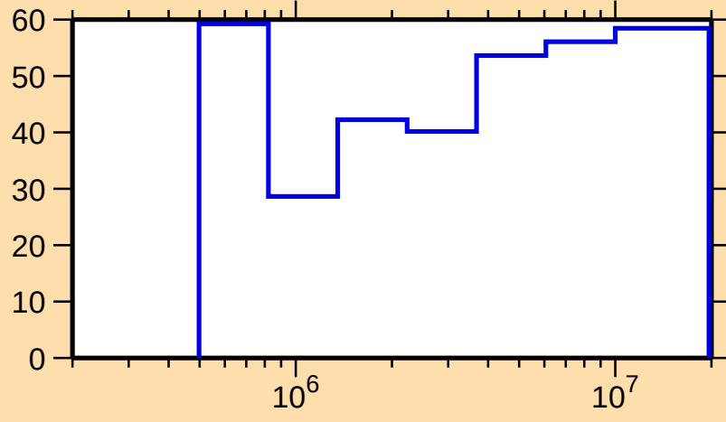
\Delta\sigma/\sigma vs. E for ^{185}\text{W}(n,n_1)
