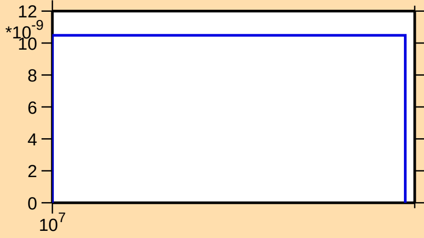
\sigma vs. E for ^{185}\text{W}(\text{n},\text{nd})
