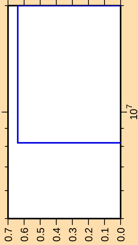
\Delta\sigma/\sigma vs. E for ^{185}\text{W}(n,\text{He3})
