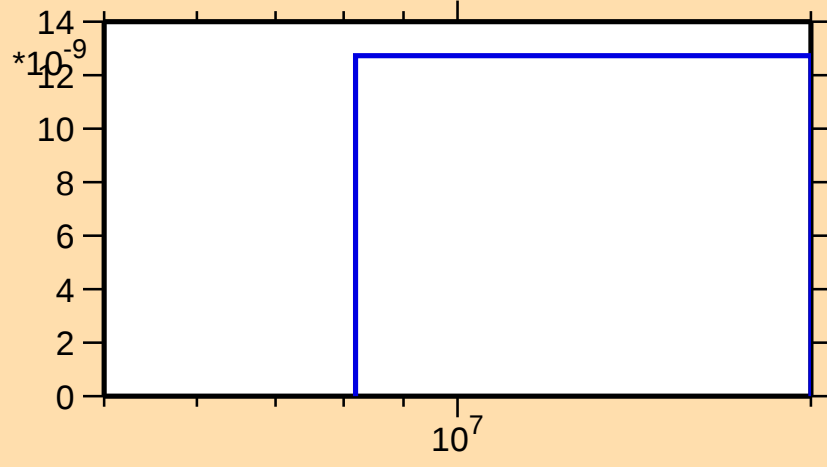
\sigma vs. E for ^{185}\text{W}(n,2n\alpha)
