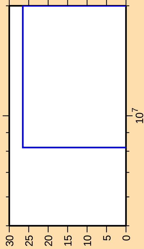
\Delta\sigma/\sigma vs. E for ^{185}\text{W}(n,3n)
