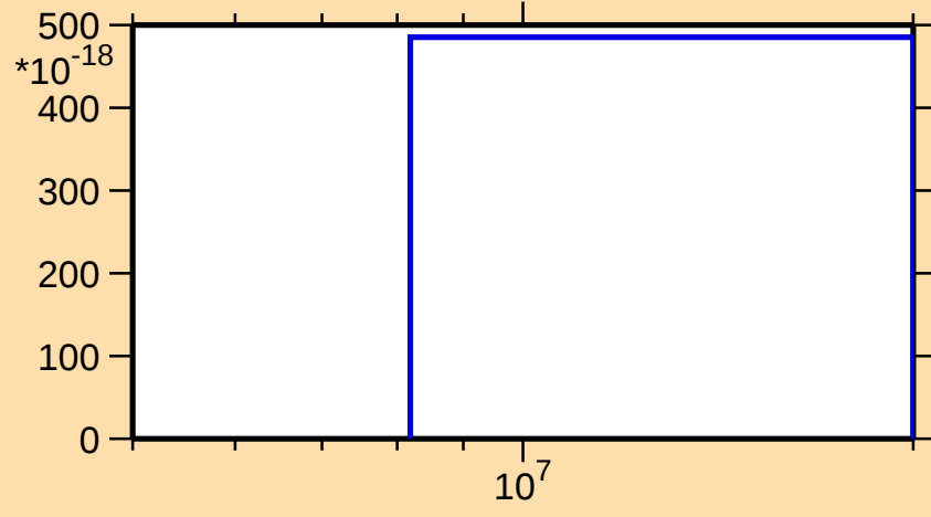
\sigma vs. E for ^{185}\text{W}(n,3n\alpha)
