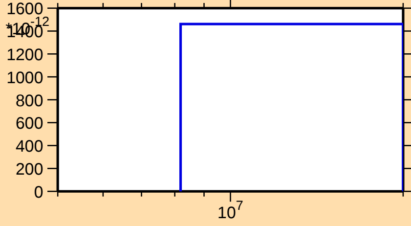
\sigma vs. E for ^{185}\text{W}(n,nt)
