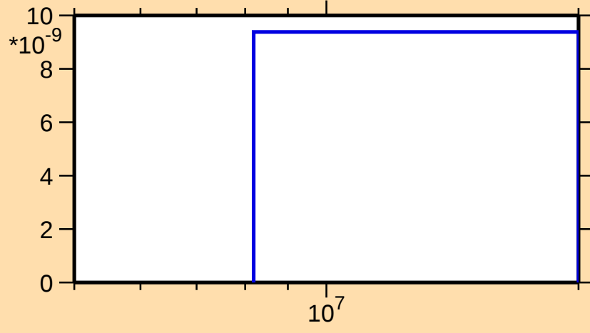
\sigma vs. E for ^{185}\text{W}(n,\text{nd})
