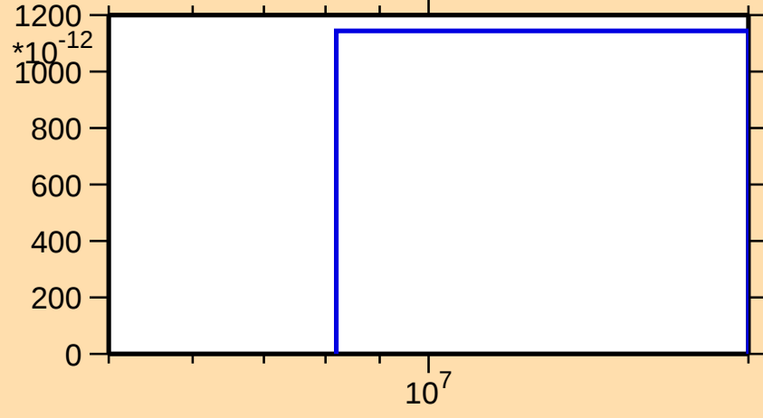
\sigma vs. E for ^{185}\text{W}(n,2np)
