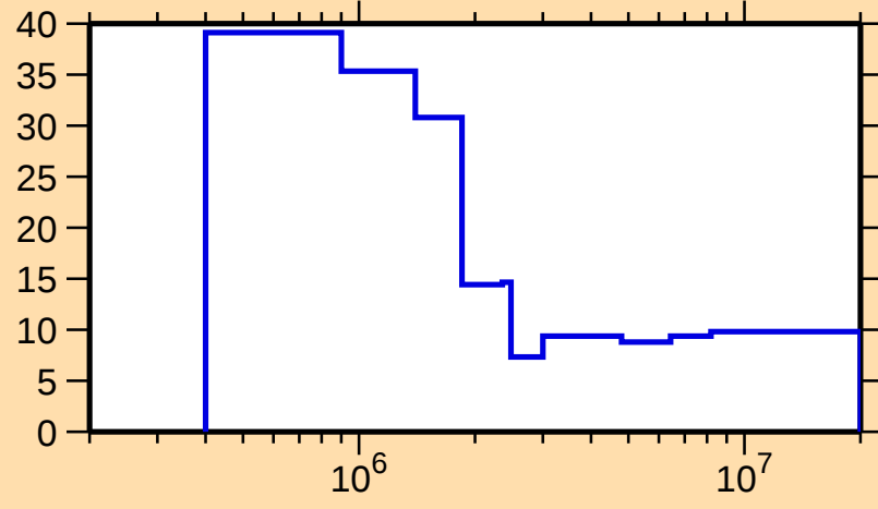
\Delta\sigma/\sigma vs. E for ^{185}\text{W}(\text{n},\text{nonel.})
