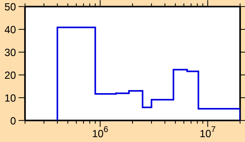
\Delta\sigma/\sigma vs. E for ^{185}\text{W}(n,\text{el.})
