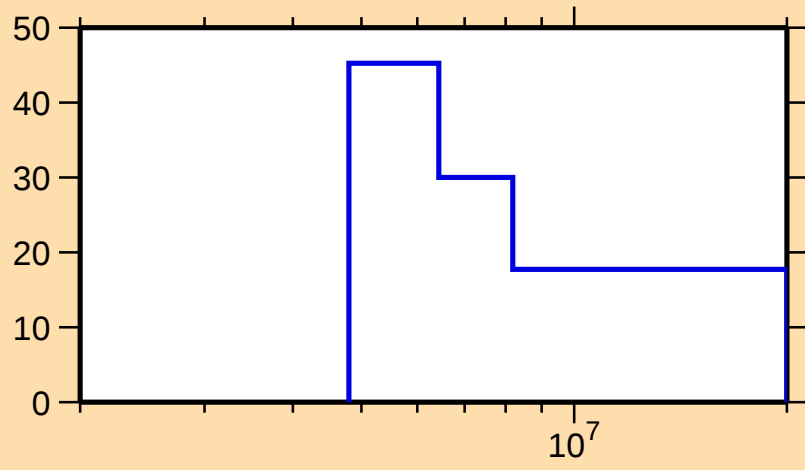
\Delta\sigma/\sigma vs. E for ^{185}\text{W}(n,2n)
