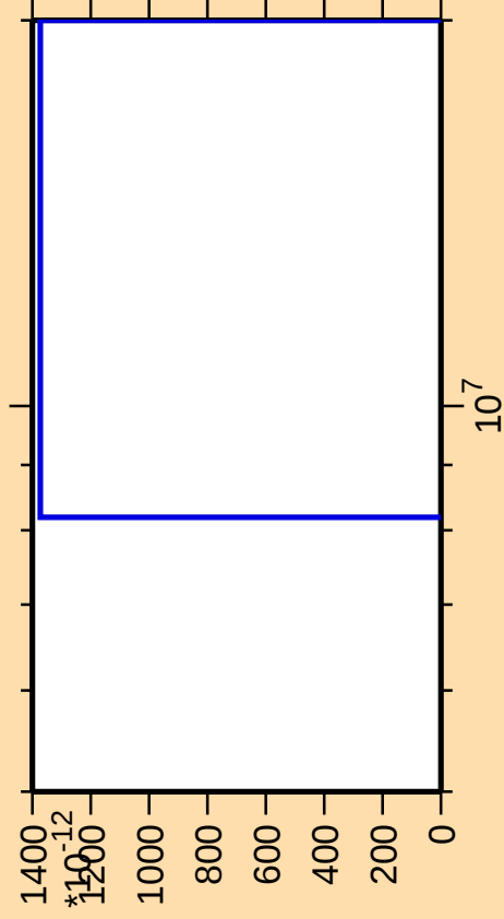
\Delta\sigma/\sigma vs. E for ^{185}\text{W}(\text{mt 11})
