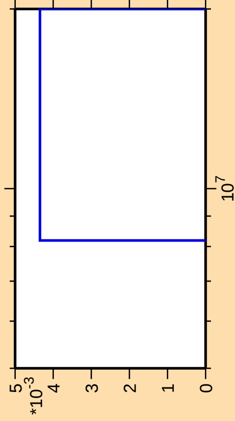
\Delta\sigma/\sigma vs. E for ^{185}\text{W}(n,3n\alpha)
