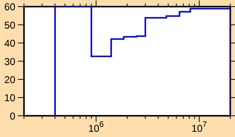
\Delta\sigma/\sigma vs. E for ^{185}\text{W}(n,n_1)
