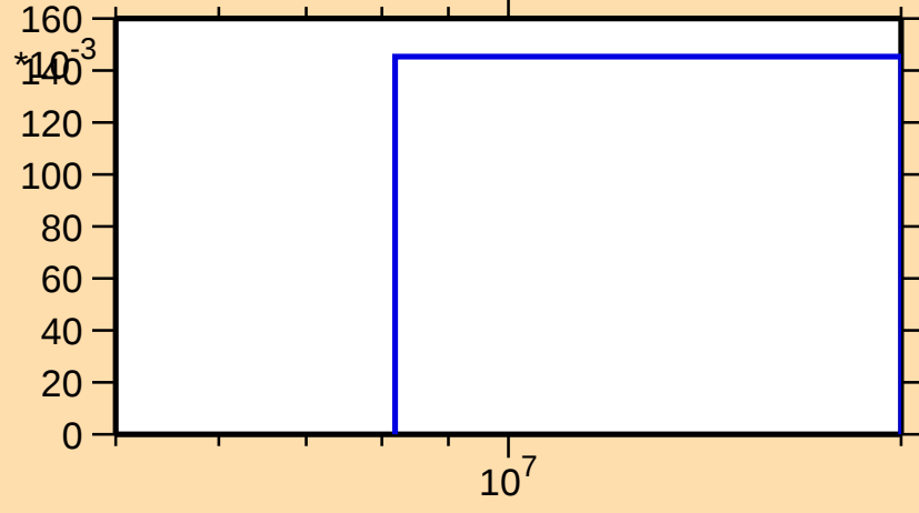
\sigma vs. E for ^{185}\text{W}(n,3n)
