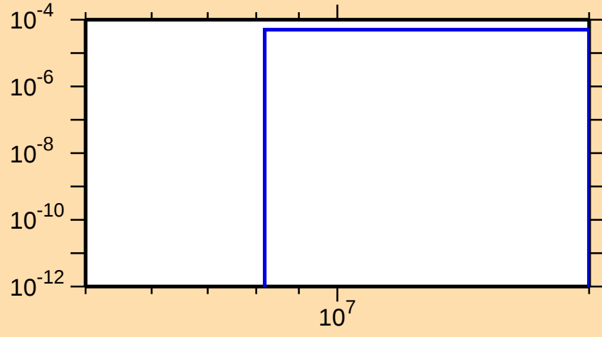
\sigma vs. E for ^{185}\text{W}(n,np)
