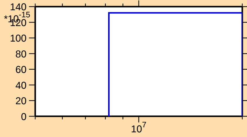
\sigma vs. E for ^{185}\text{W}(n,\text{He3})
