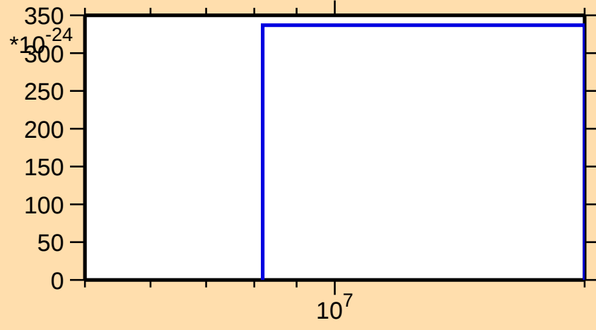
\sigma vs. E for ^{185}\text{W}(\text{mt 11})
