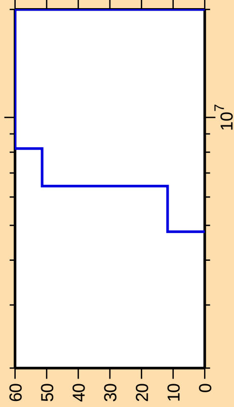
\Delta\sigma/\sigma vs. E for ^{185}\text{W}(n,n\text{cont.})
