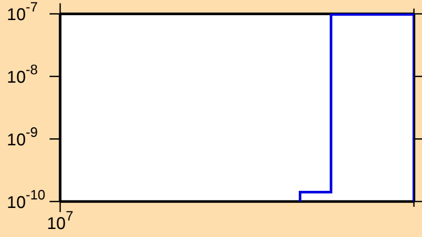
\sigma vs. E for ^{186}\text{W}(n,\text{nt})
