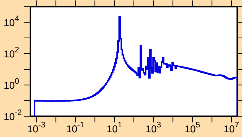
\sigma vs. E for ^{186}\text{W}(\text{n},\text{el.})
