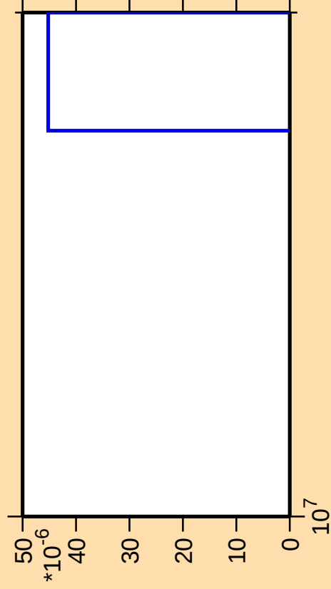
\Delta\sigma/\sigma vs. E for ^{186}\text{W} (mt 11)
