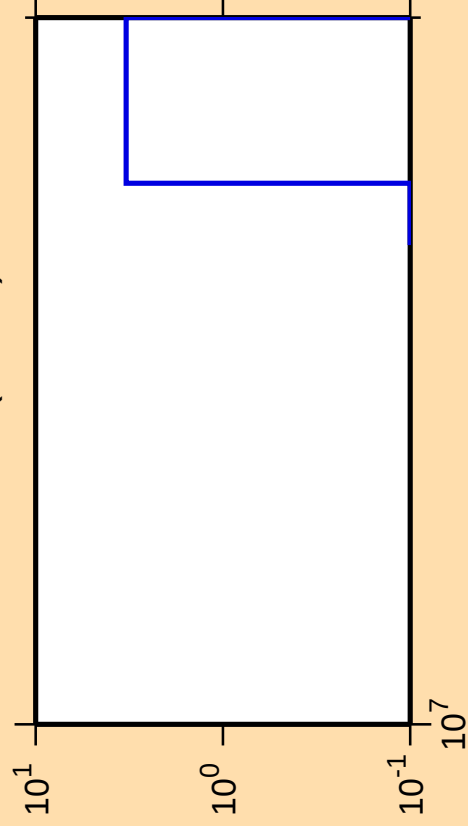
\Delta\sigma/\sigma vs. E for ^{186}\text{W}(n,\text{He3})
