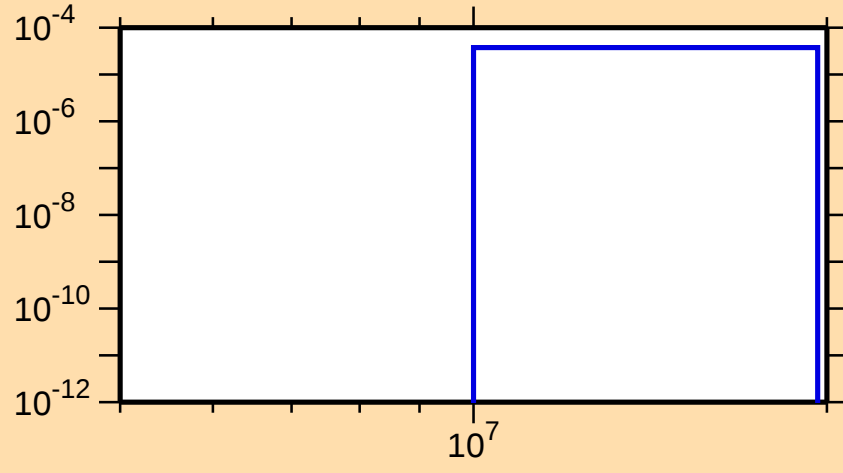
\sigma vs. E for ^{186}\text{W}(n,np)
