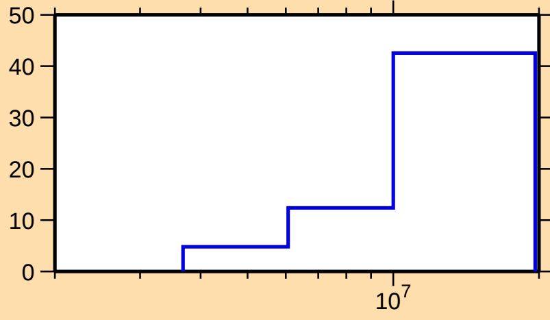
\Delta\sigma/\sigma vs. E for ^{186}\text{W}(n,n\text{cont.})
