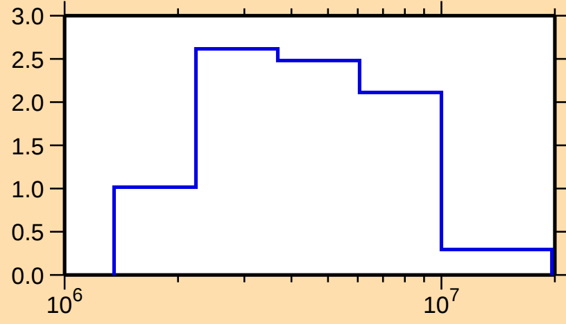
\sigma vs. E for ^{186}\text{W}(n,n\text{cont.})
