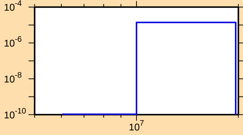
\sigma vs. E for ^{186}\text{W}(n,n\alpha)
