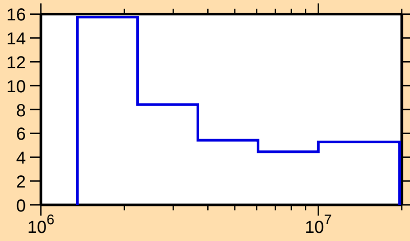
\Delta\sigma/\sigma vs. E for ^{186}\text{W}(\text{n},\text{nonel.})
