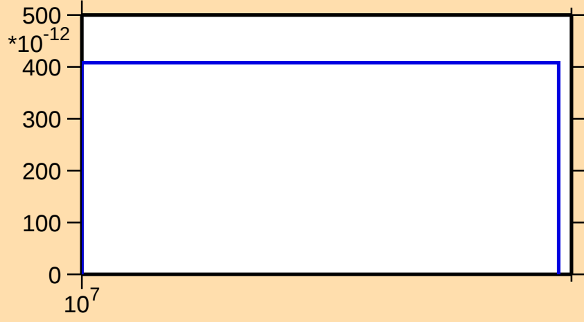
\sigma vs. E for ^{186}\text{W}(\text{n},\text{nd})
