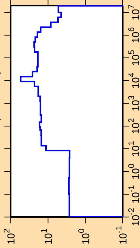
\Delta\sigma/\sigma vs. E for ^{186}\text{W}(n,\text{nonel.})
