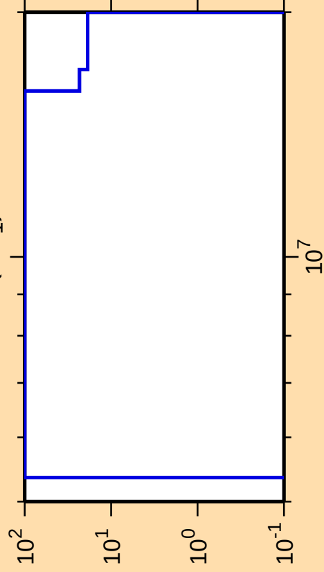
\Delta\sigma/\sigma vs. E for ^{187}\text{W}(n,n_1)
