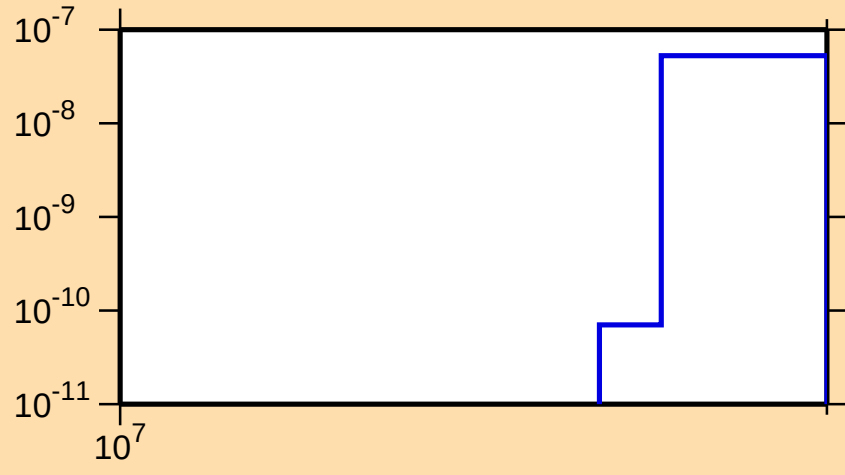
\sigma vs. E for ^{187}\text{W}(n,2np)
