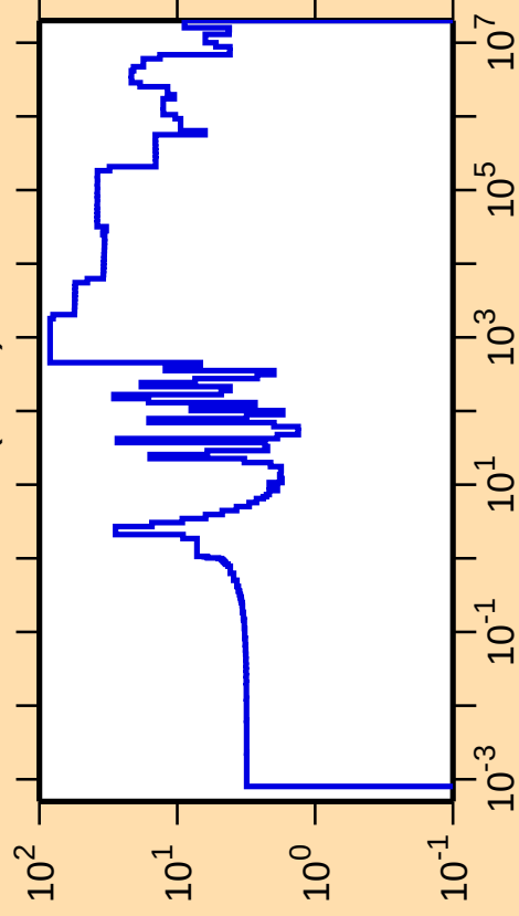
\Delta\sigma/\sigma vs. E for ^{187}\text{W}(\text{n,el.})
