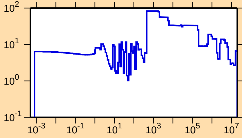
\Delta\sigma/\sigma vs. E for ^{187}\text{W}(\text{n,tot.})
