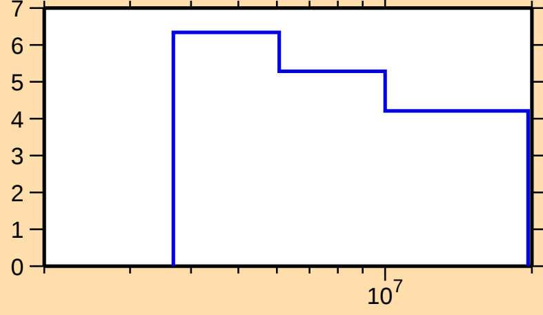
\Delta\sigma/\sigma vs. E for ^{187}\text{W}(n,\text{nonel.})
