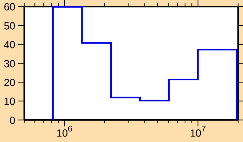
\Delta\sigma/\sigma vs. E for ^{187}\text{W}(n,n\text{cont.})
