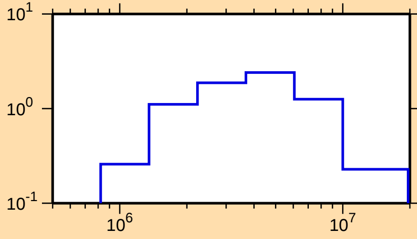
\sigma vs. E for ^{187}\text{W}(n,n\text{cont.})
