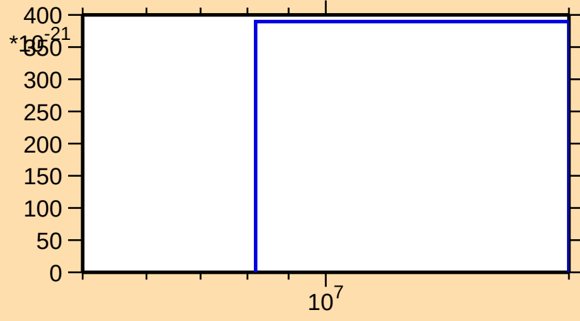
\sigma vs. E for ^{187}\text{W}(\text{mt } 11)
