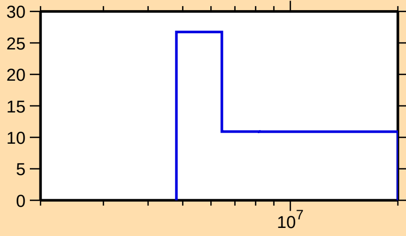
\Delta\sigma/\sigma vs. E for ^{187}\text{W}(n,2n)
