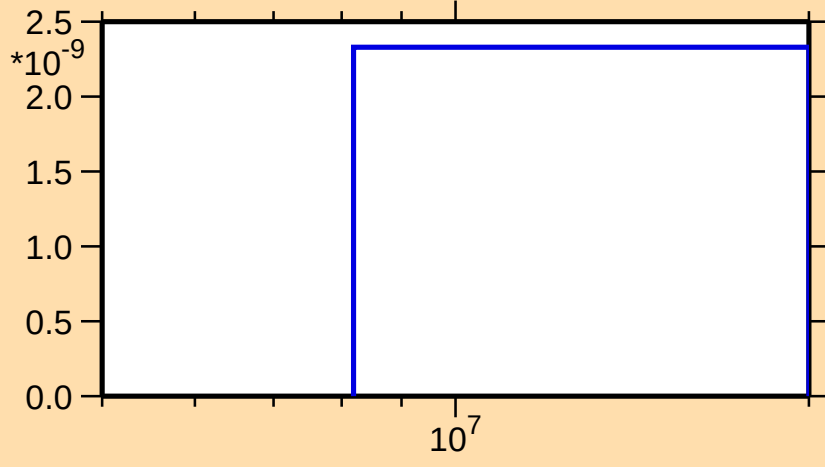
\sigma vs. E for ^{187}\text{W}(n,2n\alpha)
