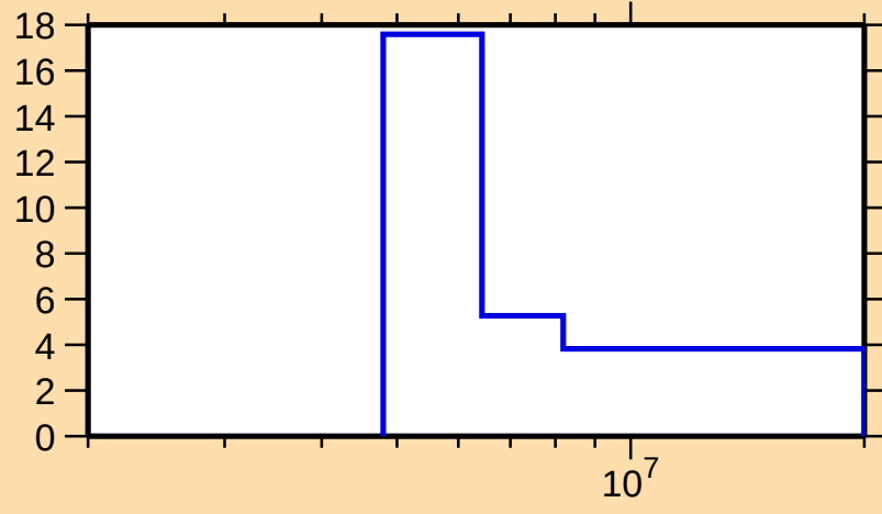
\Delta\sigma/\sigma vs. E for ^{187}\text{W}(n,\text{el.})
