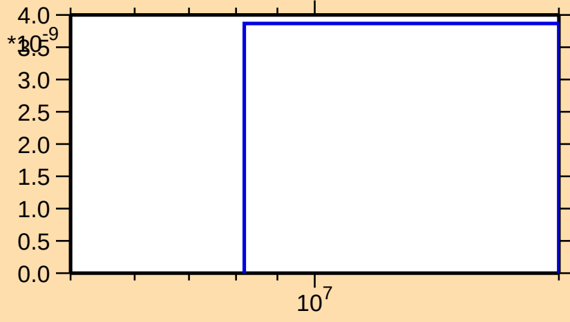
\sigma vs. E for ^{187}\text{W}(\text{n},\text{nd})
