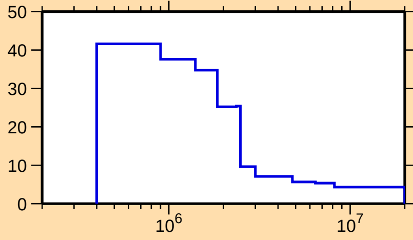
\Delta\sigma/\sigma vs. E for ^{187}\text{W}(\text{n},\text{nonel.})
