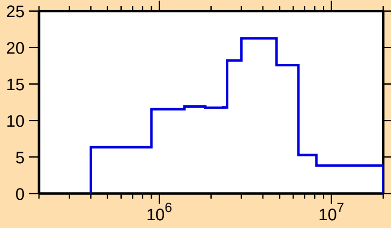
\Delta\sigma/\sigma vs. E for ^{187}\text{W}(\text{n},\text{el.})
