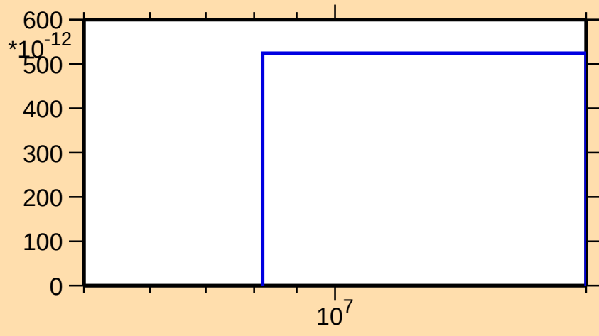
\sigma vs. E for ^{187}\text{W}(n,nt)
