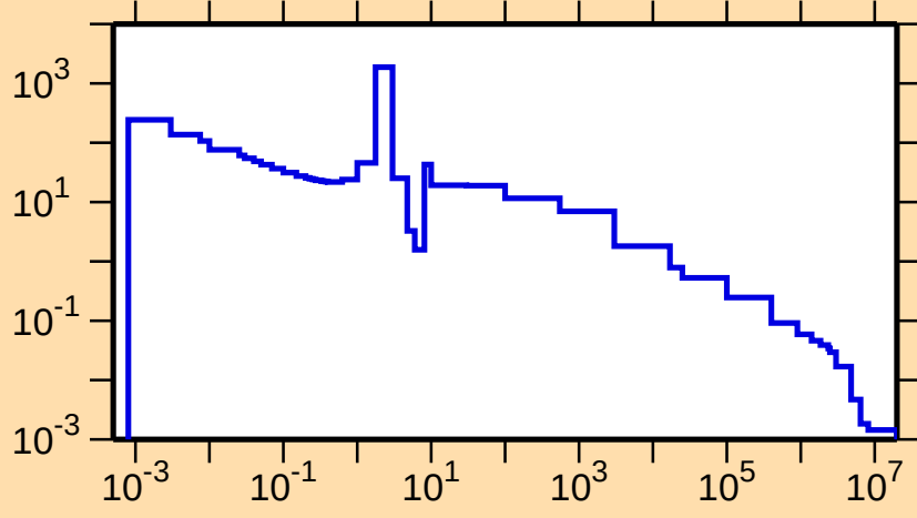
\sigma vs. E for ^{187}\text{W}(n,\gamma)
