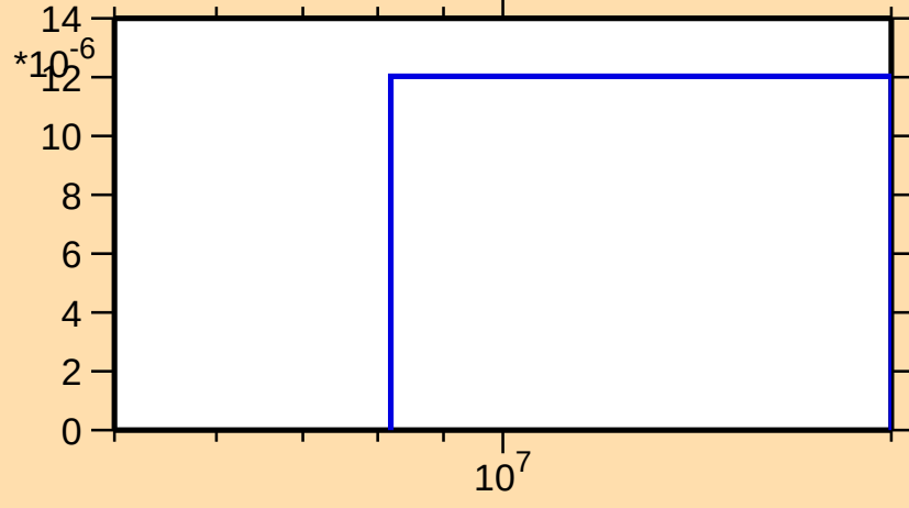
\sigma vs. E for ^{187}\text{W}(n,t)
