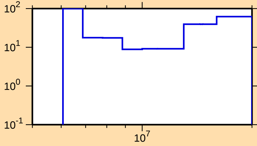
\Delta\sigma/\sigma vs. E for ^{188}\text{W}(n,2n)
