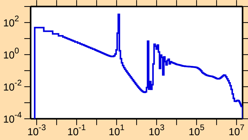
\sigma vs. E for ^{188}\text{W}(n,\gamma)
