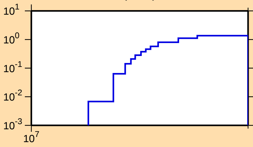
\sigma vs. E for ^{188}\text{W}(n,3n)
