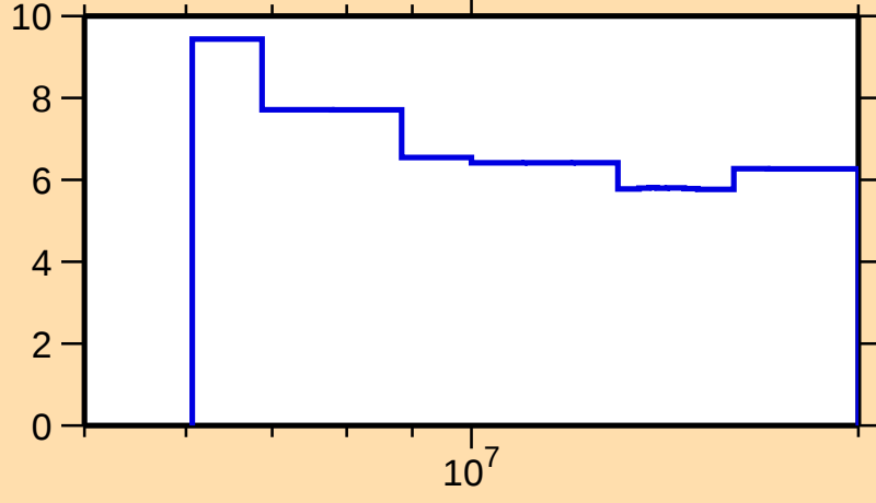
\Delta\sigma/\sigma vs. E for ^{188}\text{W}(n,\text{nonel.})
