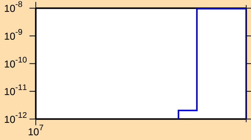
\sigma vs. E for ^{188}\text{W}(n,\text{nd})
