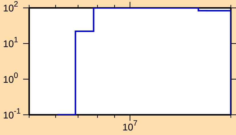
\Delta\sigma/\sigma vs. E for ^{188}\text{W}(n,p)
