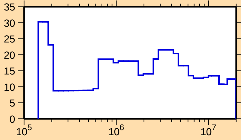
\Delta\sigma/\sigma vs. E for ^{188}\text{W}(n,\text{el.})
