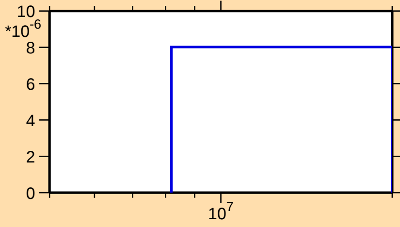
\sigma vs. E for ^{188}\text{W}(n,np)
