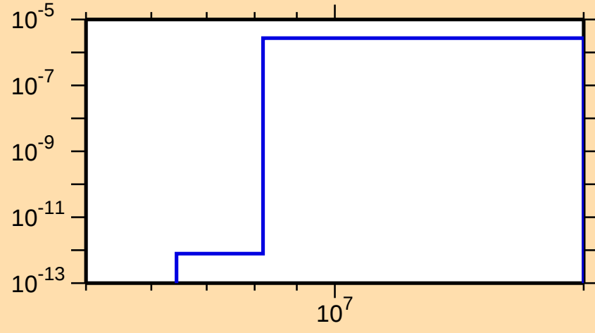
\sigma vs. E for ^{188}\text{W}(n,n\alpha)
