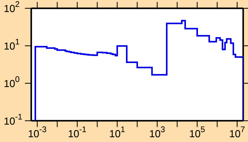
\Delta\sigma/\sigma vs. E for ^{188}\text{W}(n,\text{tot.})
