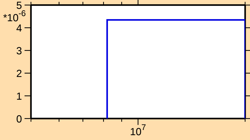
\sigma vs. E for ^{188}\text{W}(n,t)
