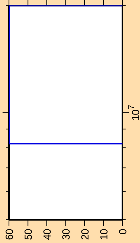
\Delta\sigma/\sigma vs. E for ^{188}\text{W}(n,\text{nt})
