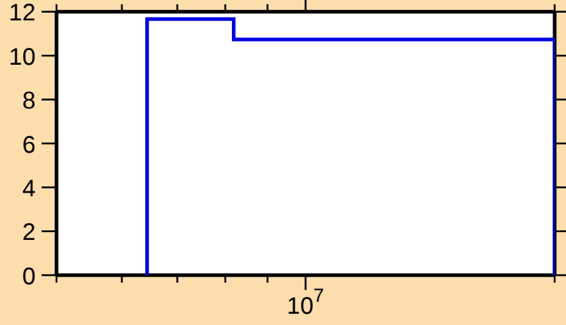
\Delta\sigma/\sigma vs. E for ^{188}\text{W}(n,\text{el.})
