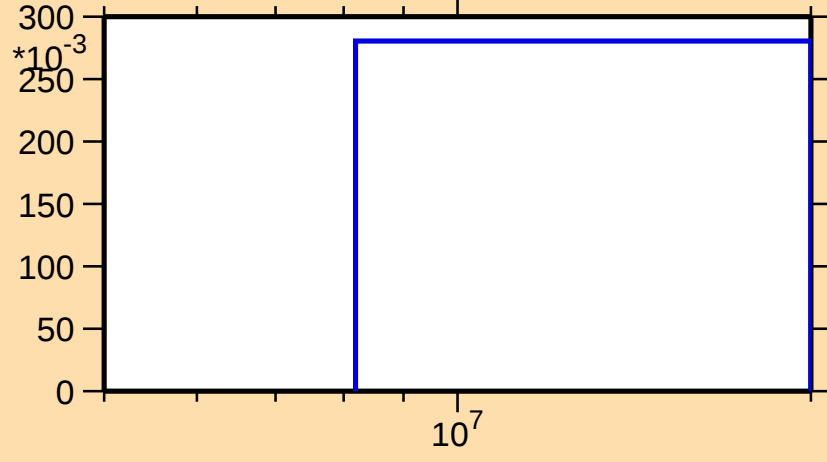
\sigma vs. E for ^{188}\text{W}(n,3n)
