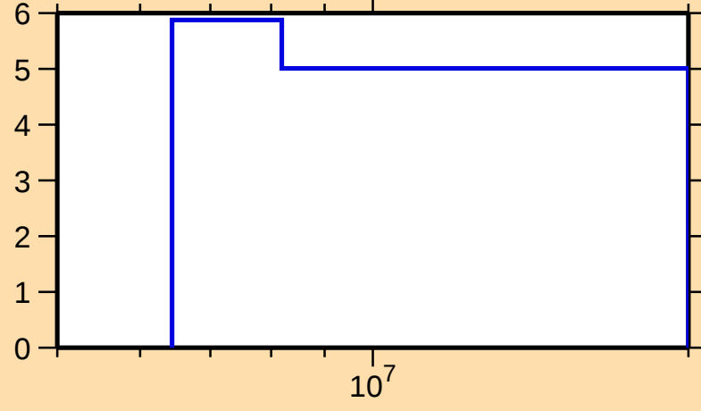
\Delta\sigma/\sigma vs. E for ^{188}\text{W}(n,\text{tot.})
