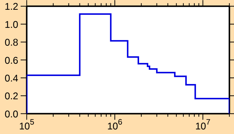
\sigma vs. E for ^{188}\text{W}(n,n_1)
