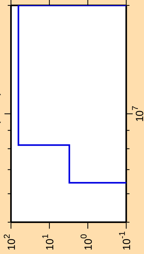
\Delta\sigma/\sigma vs. E for ^{188}\text{W}(n,n\alpha)
