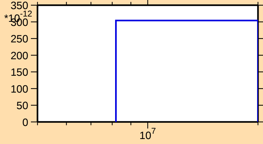
\sigma vs. E for ^{188}\text{W}(n,\text{nt})
