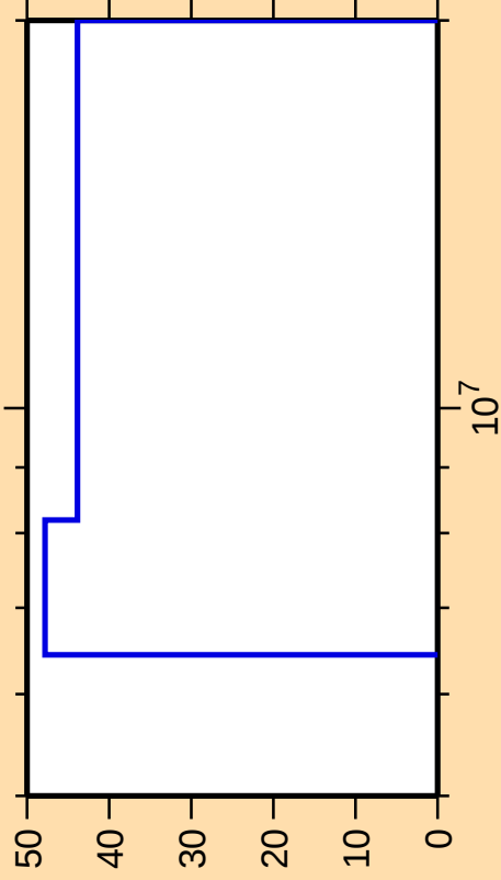
\Delta\sigma/\sigma vs. E for ^{188}\text{W}(n,n_1)
