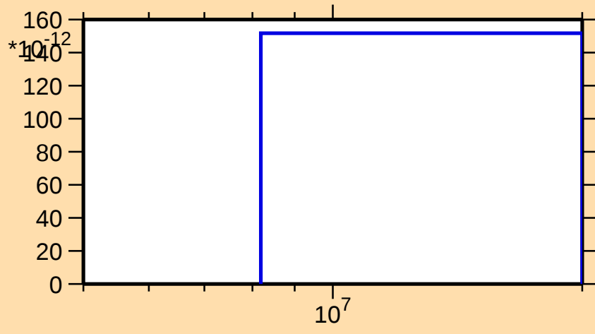
\sigma vs. E for ^{188}\text{W}(n,2n\alpha)
