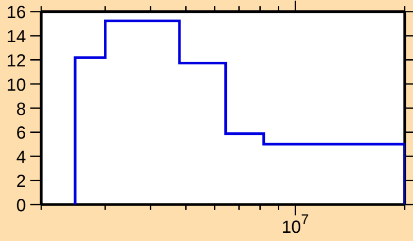
\Delta\sigma/\sigma vs. E for ^{188}\text{W}(n,\text{tot.})
