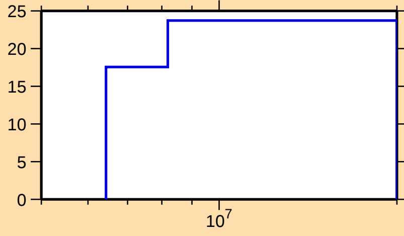
\Delta\sigma/\sigma vs. E for ^{188}\text{W}(n,2n)
