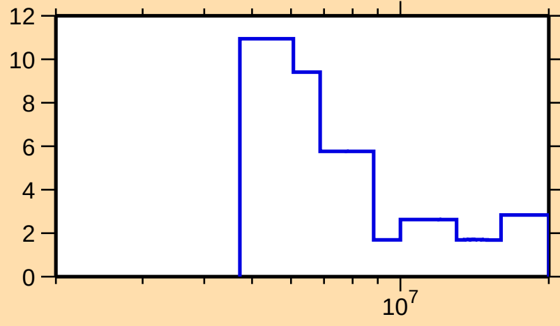
\Delta\sigma/\sigma vs. E for ^{189}\text{W}(n,\text{tot.})
