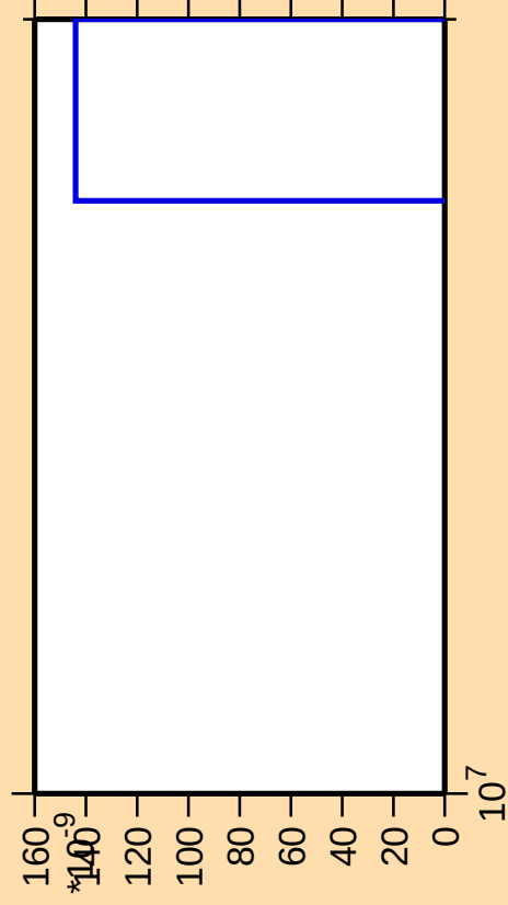
\Delta\sigma/\sigma vs. E for ^{189}\text{W}(\text{mt } 11)
