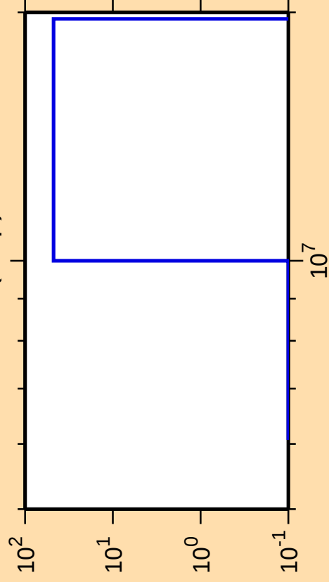
\Delta\sigma/\sigma vs. E for ^{189}\text{W}(n,np)
