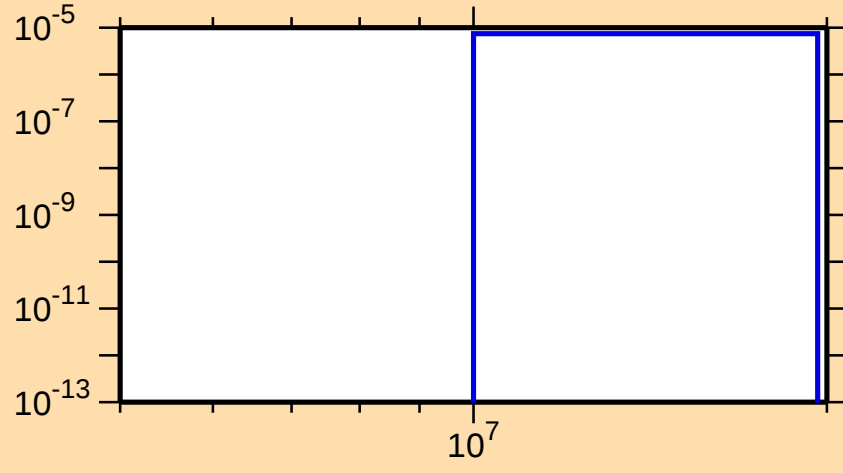
\sigma vs. E for ^{189}\text{W}(n,np)
