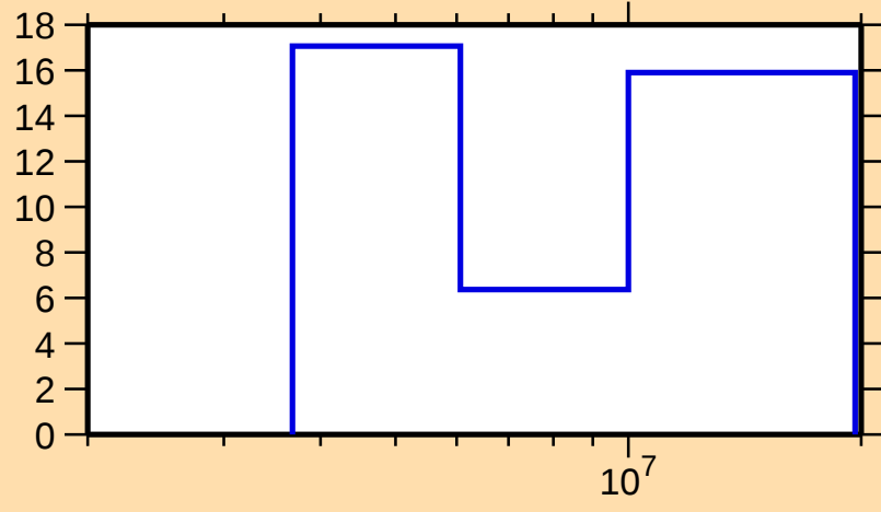
\Delta\sigma/\sigma vs. E for ^{189}\text{W}(n,2n)
