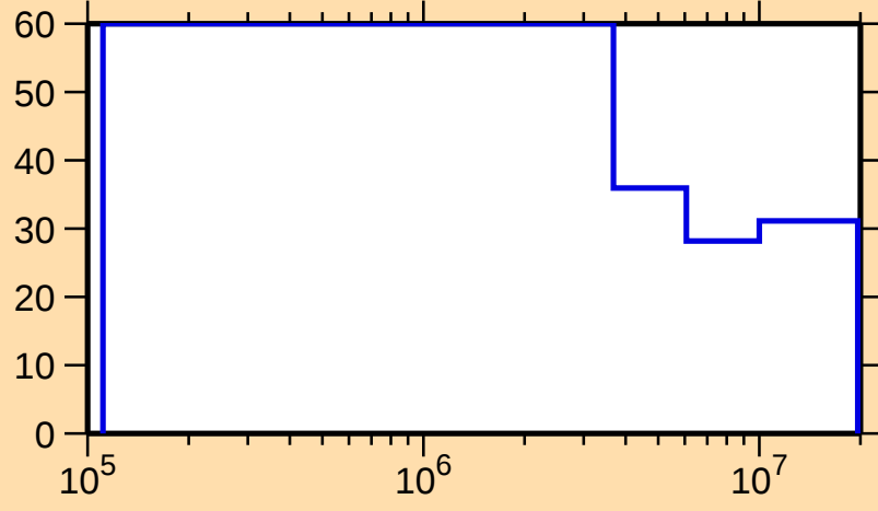
\Delta\sigma/\sigma vs. E for ^{189}\text{W}(n,n_1)
