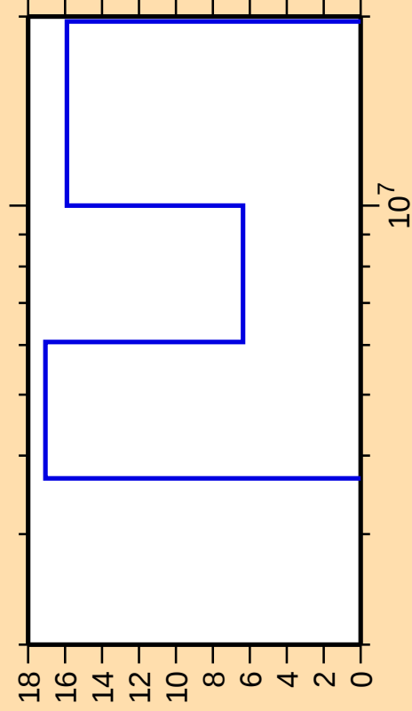
\Delta\sigma/\sigma vs. E for ^{189}\text{W}(n,2n)
