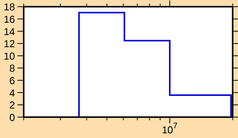
\Delta\sigma/\sigma vs. E for ^{189}\text{W}(n,\text{el.})
