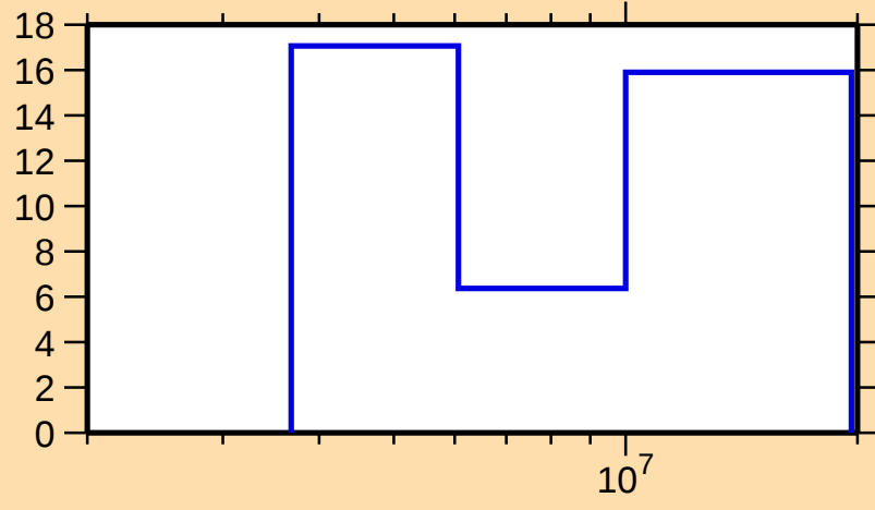
\Delta\sigma/\sigma vs. E for ^{189}\text{W}(n,2n)
