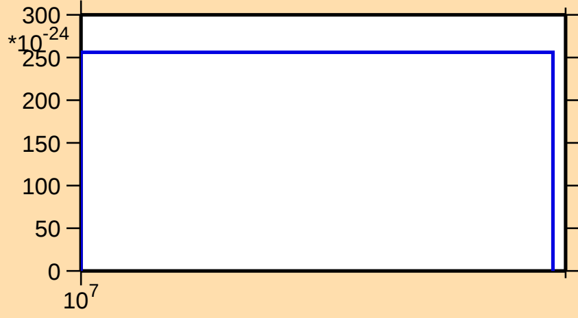
\sigma vs. E for ^{189}\text{W}(\text{mt 11})
