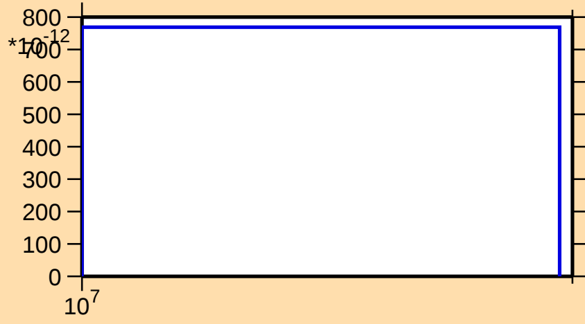
\sigma vs. E for ^{189}\text{W}(n,nt)
