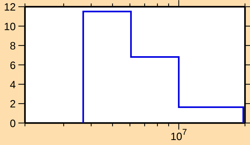
\Delta\sigma/\sigma vs. E for ^{189}\text{W}(n,\text{tot.})
