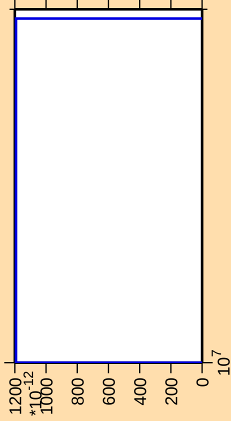
\Delta\sigma/\sigma vs. E for ^{189}\text{W}(\text{mt 11})
