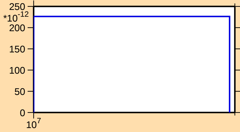
\sigma vs. E for ^{189}\text{W}(n,2np)
