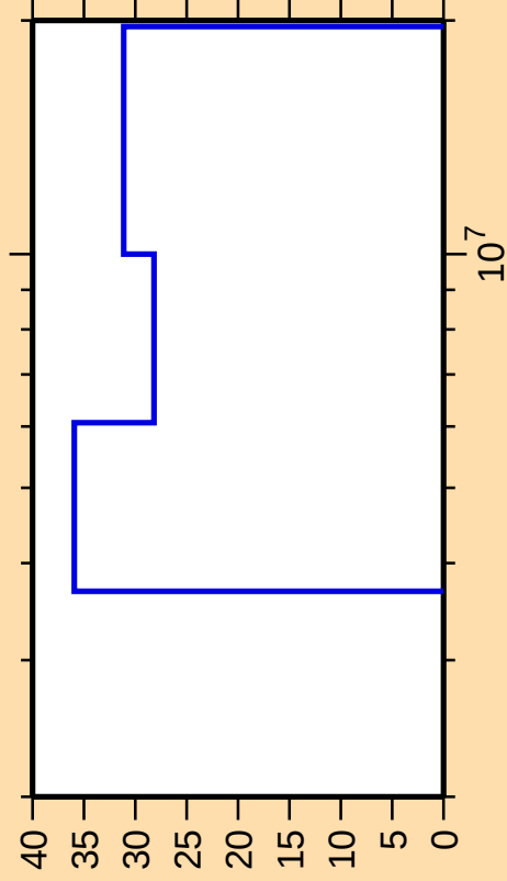
\Delta\sigma/\sigma vs. E for ^{189}\text{W}(n,n_1)
