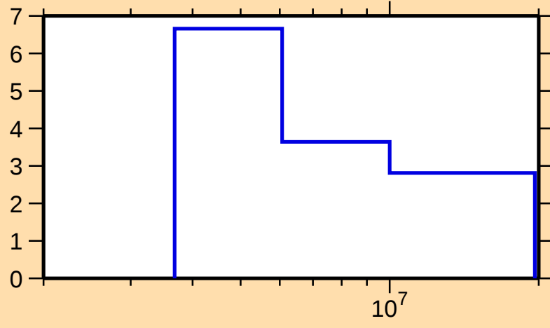
\Delta\sigma/\sigma vs. E for ^{189}\text{W}(n,\text{nonel.})
