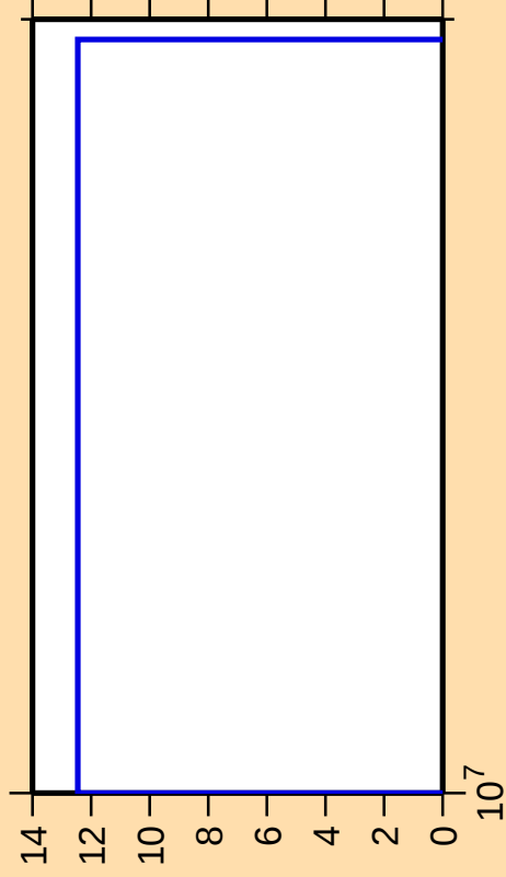
\Delta\sigma/\sigma vs. E for ^{189}\text{W}(n,3n)
