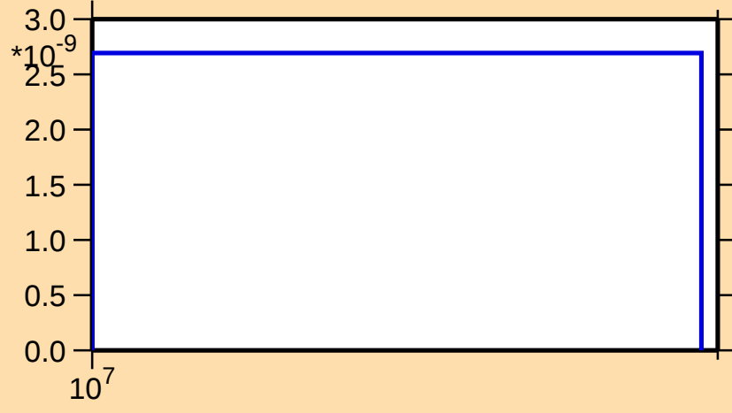
\sigma vs. E for ^{189}\text{W}(\text{n},\text{nd})
