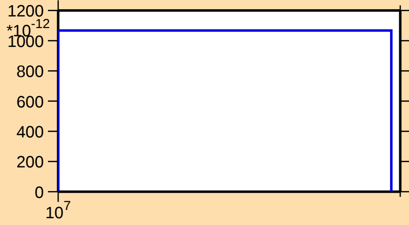
\sigma vs. E for ^{189}\text{W}(n,2n\alpha)
