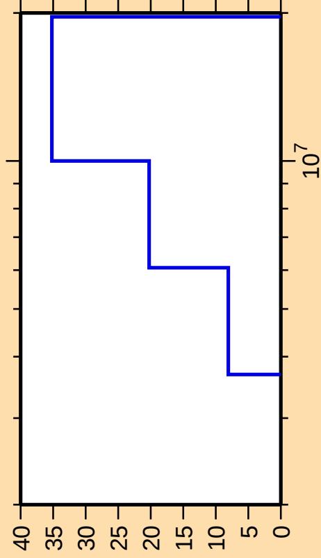
\Delta\sigma/\sigma vs. E for ^{189}\text{W}(n,n\text{cont.})
