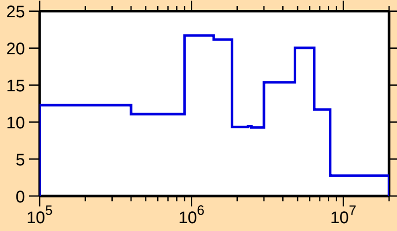
\Delta\sigma/\sigma vs. E for ^{189}\text{W}(n,\text{el.})
