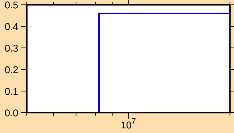
\sigma vs. E for ^{189}\text{W}(n,3n)
