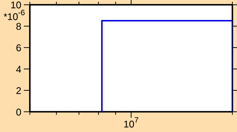
\sigma vs. E for ^{189}\text{W}(n,t)
