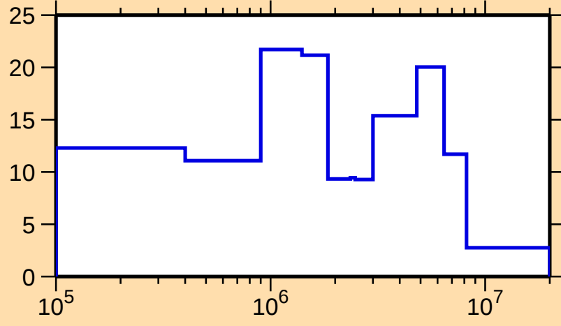
\Delta\sigma/\sigma vs. E for ^{189}\text{W}(\text{n},\text{el.})
