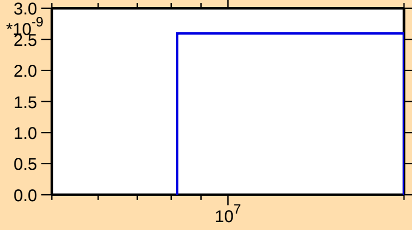
\sigma vs. E for ^{189}\text{W}(n,\text{nd})
