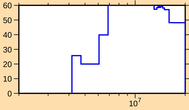
\Delta\sigma/\sigma vs. E for ^{190}\text{W}(n,n\text{cont.})
