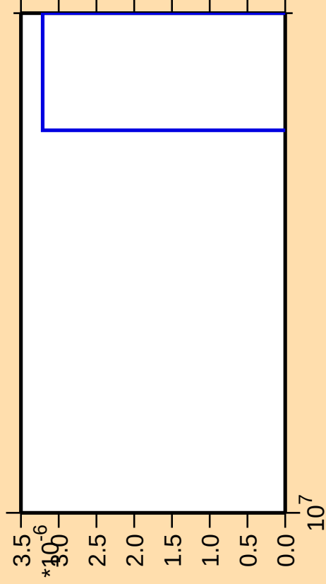
\Delta\sigma/\sigma vs. E for ^{190}\text{W}(\text{mt 11})
