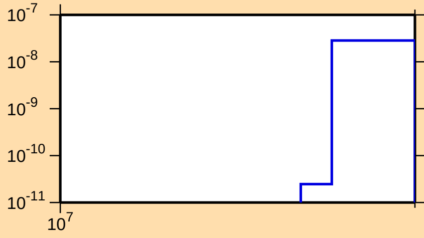
\sigma vs. E for ^{190}\text{W}(n,nt)
