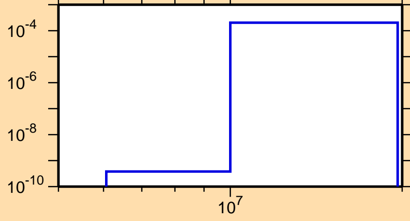
\sigma vs. E for ^{190}\text{W}(n,p)
