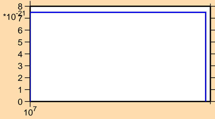
\sigma vs. E for ^{190}\text{W} (mt 11)
