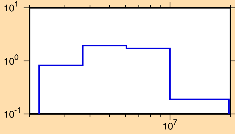
\sigma vs. E for ^{190}\text{W}(n,n\text{cont.})
