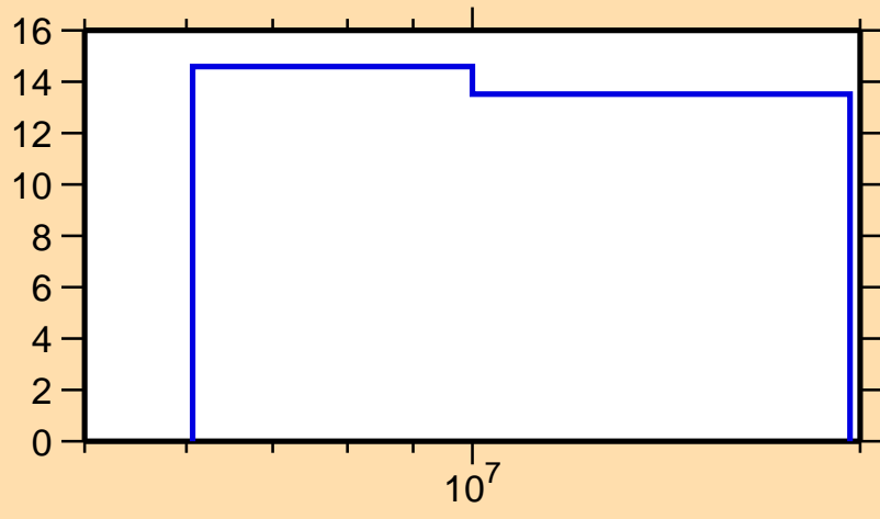
\Delta\sigma/\sigma vs. E for ^{190}\text{W}(n,\text{nonel.})
