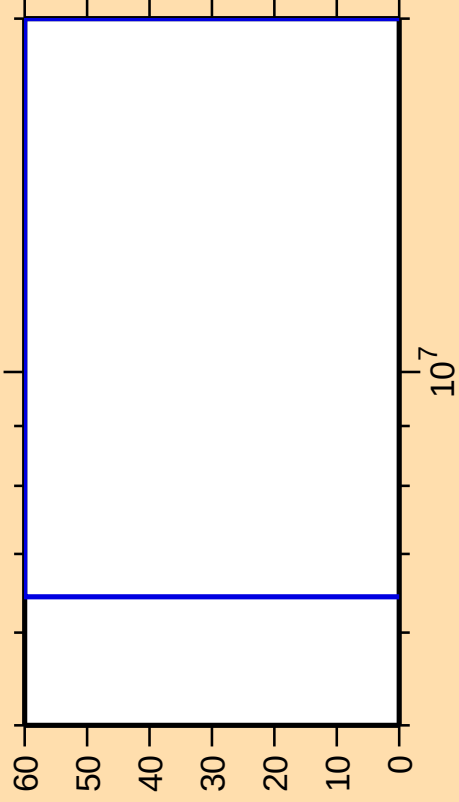
\Delta\sigma/\sigma vs. E for ^{190}\text{W}(n,n\text{cont.})
