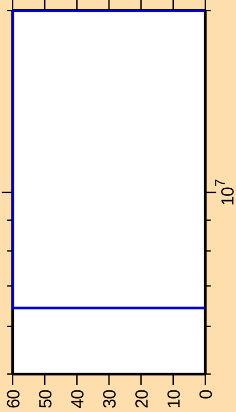
\Delta\sigma/\sigma vs. E for ^{190}\text{W}(n,\gamma)
