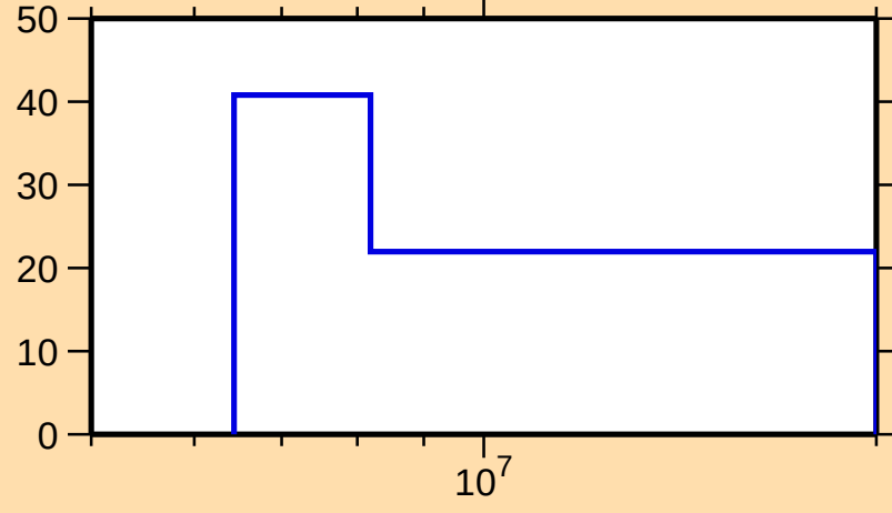
\Delta\sigma/\sigma vs. E for ^{190}\text{W}(n,2n)
