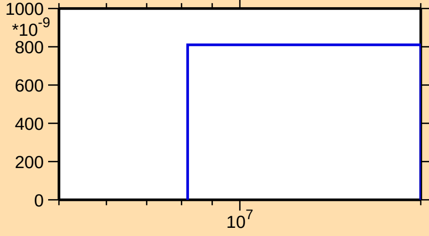
\sigma vs. E for ^{190}\text{W}(n,n\alpha)
