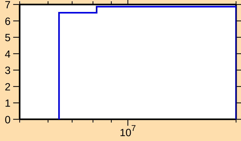
\Delta\sigma/\sigma vs. E for ^{190}\text{W}(n,\text{tot.})
