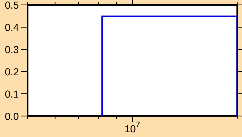
\sigma vs. E for ^{190}\text{W}(n,3n)
