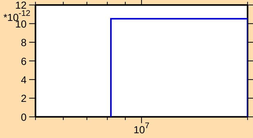
\sigma vs. E for ^{190}\text{W}(n,\text{nd})
