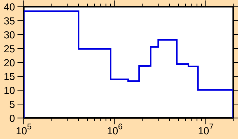
\Delta\sigma/\sigma vs. E for ^{190}\text{W}(n,\text{el.})
