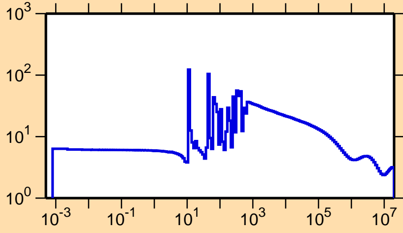
\sigma vs. E for ^{191}\text{W}(n,\text{el.})
