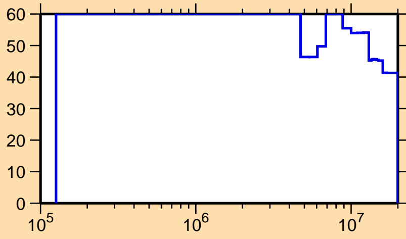
\Delta\sigma/\sigma vs. E for ^{191}\text{W}(n,n_1)
