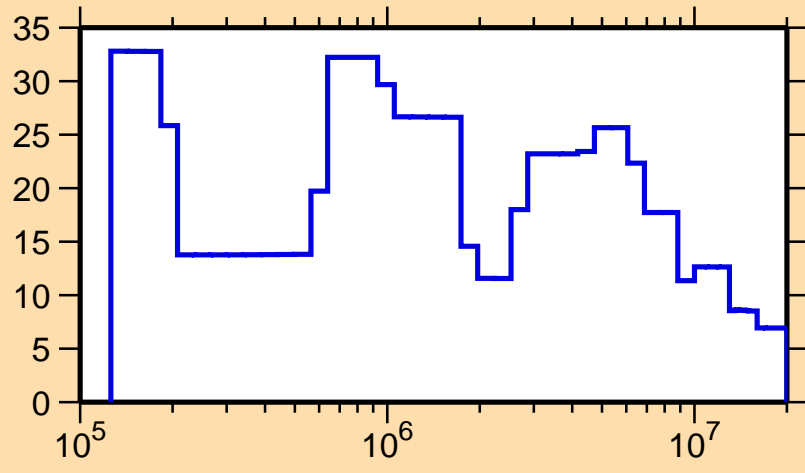
\Delta\sigma/\sigma vs. E for ^{191}\text{W}(n, el.)
