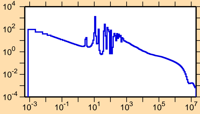
\sigma vs. E for ^{191}\text{W}(n,\gamma)
