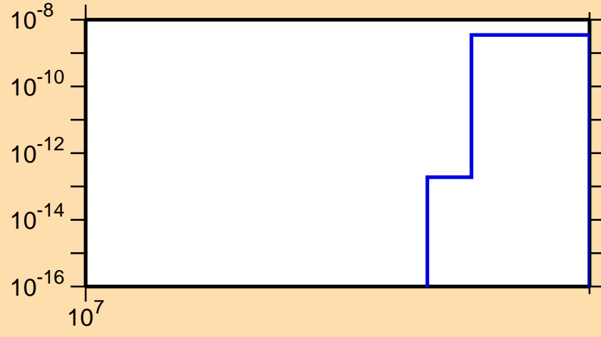
\sigma vs. E for ^{191}\text{W}(n,2np)
