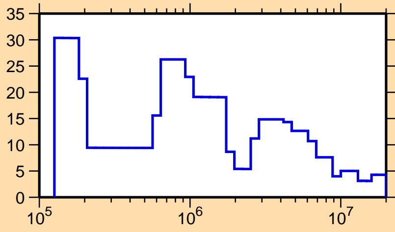
\Delta\sigma/\sigma vs. E for ^{191}\text{W}(n, tot.)
