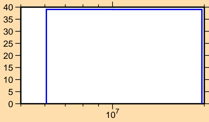
\Delta\sigma/\sigma vs. E for ^{191}\text{W}(n,p)
