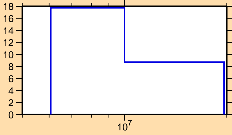
\Delta\sigma/\sigma vs. E for ^{191}\text{W}(n,el.)
