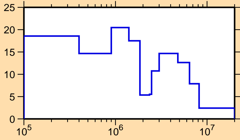
\Delta\sigma/\sigma vs. E for ^{191}\text{W}(n,\text{tot.})
