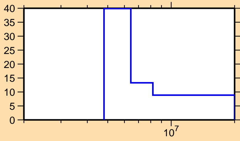
\Delta\sigma/\sigma vs. E for ^{191}\text{W}(n,2n)
