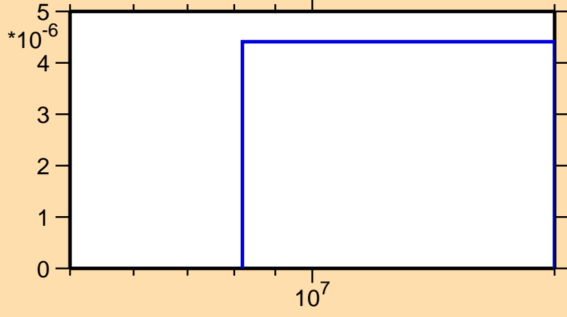
\sigma vs. E for ^{191}\text{W}(n,d)
