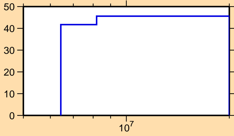
\Delta\sigma/\sigma vs. E for ^{191}\text{W}(n,ncont.)
