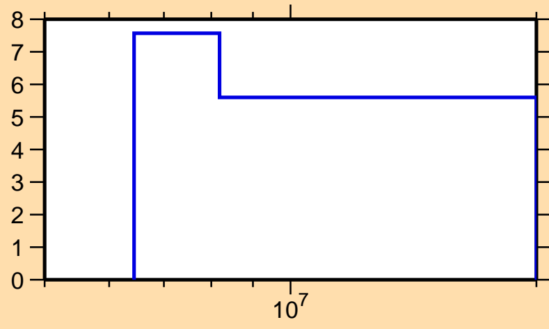
\Delta\sigma/\sigma vs. E for ^{191}\text{W}(n,\text{nonel.})
