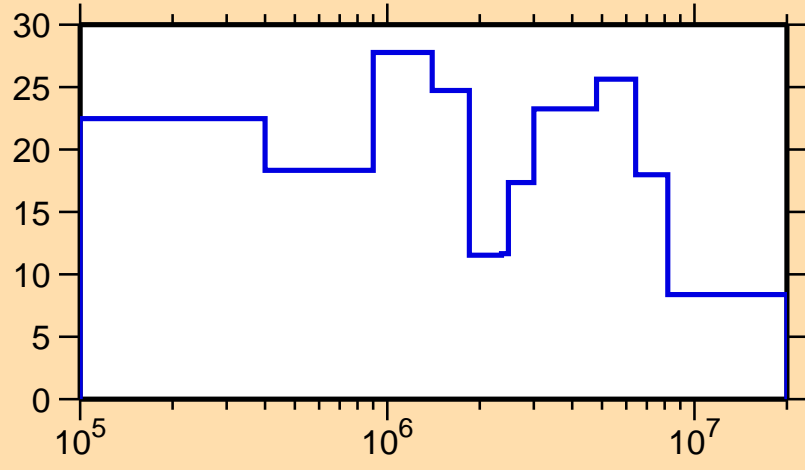
\Delta\sigma/\sigma vs. E for ^{191}\text{W}(n, \text{el.})
