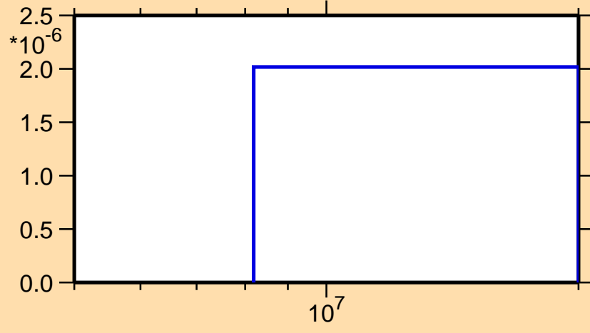
\sigma vs. E for ^{191}\text{W}(n,np)
