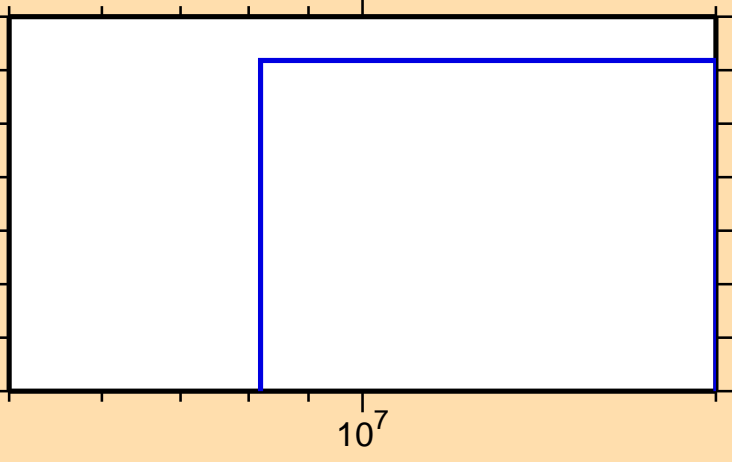
\sigma vs. E for ^{191}\text{W}(n,n\alpha)
