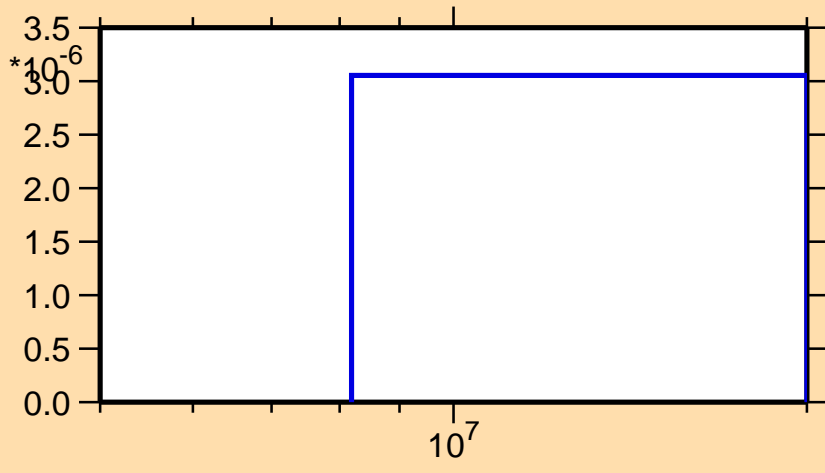
\sigma vs. E for ^{191}\text{W}(n,t)
