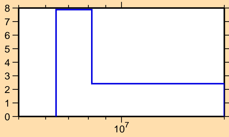
\Delta\sigma/\sigma vs. E for ^{191}\text{W}(n,\text{tot.})
