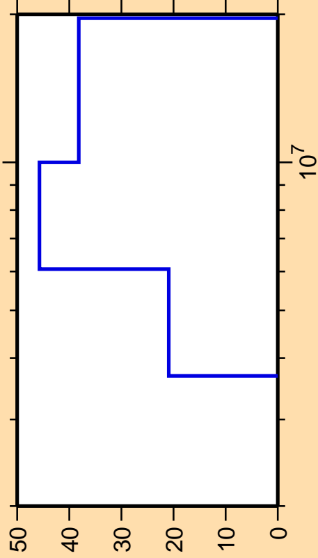
\Delta\sigma/\sigma vs. E for ^{193}\text{W}(n,n\text{cont.})
