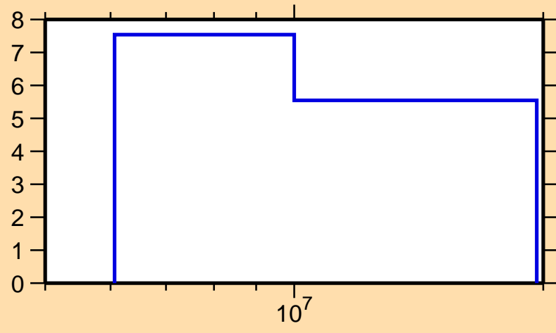
\Delta\sigma/\sigma vs. E for ^{193}\text{W}(n, \text{tot.})
