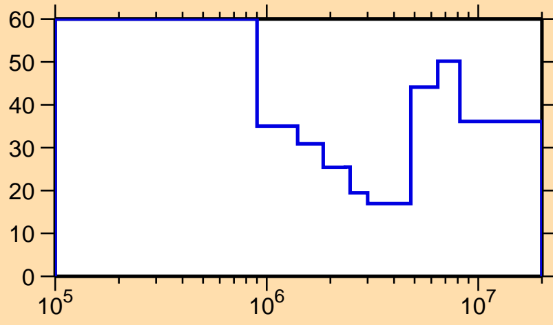
\Delta\sigma/\sigma vs. E for ^{193}\text{W}(n,n\text{cont.})
