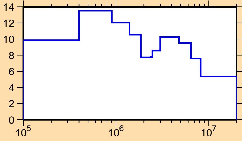
\Delta\sigma/\sigma vs. E for ^{193}\text{W}(n, tot.)
