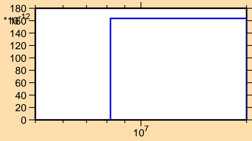
\sigma vs. E for ^{193}\text{W}(n,\text{nd})
