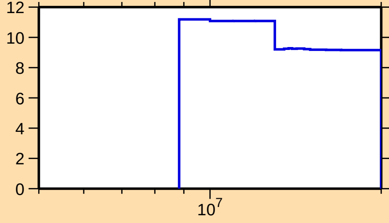
\Delta\sigma/\sigma vs. E for ^{194}\text{W}(\text{n},\text{nonel.})
