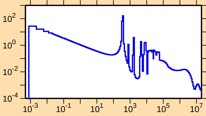
\sigma vs. E for ^{194}\text{W}(n,\gamma)
