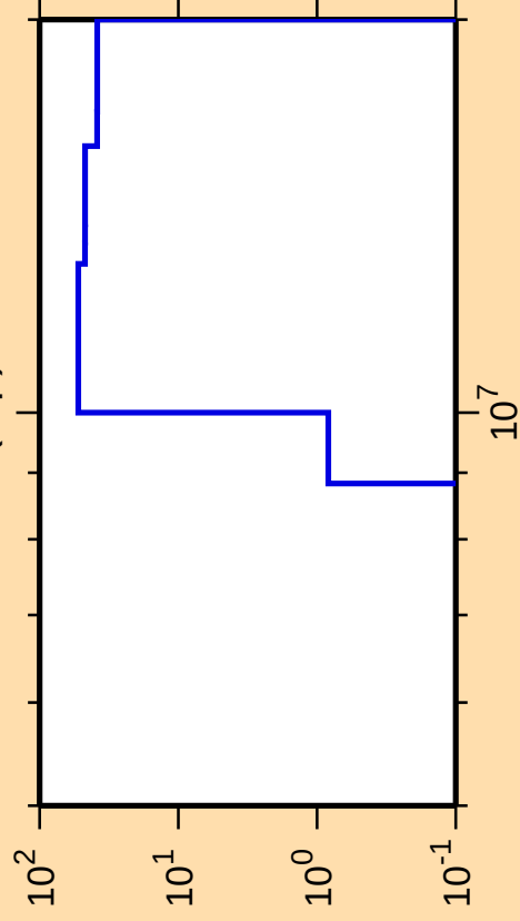
\Delta\sigma/\sigma vs. E for ^{194}\text{W}(\text{n},\text{p})
