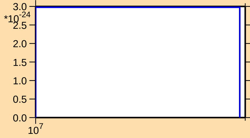
\sigma vs. E for ^{194}\text{W}(\text{mt 11})
