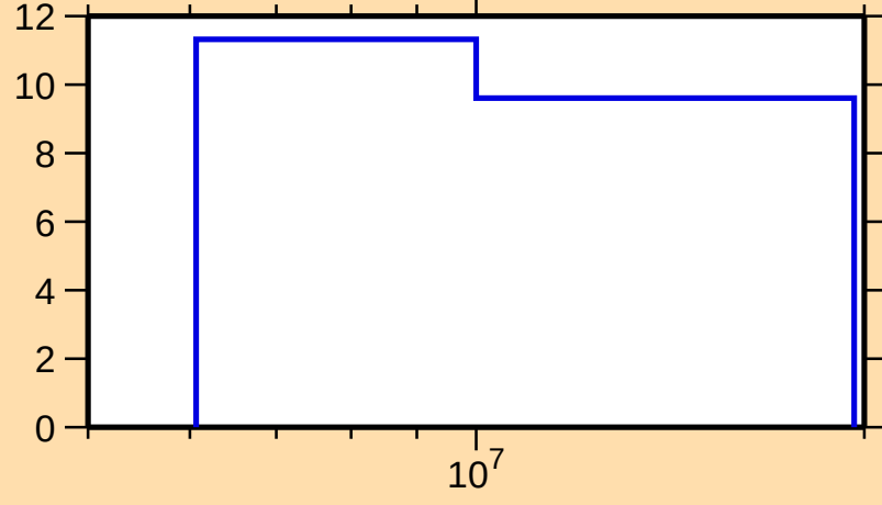
\Delta\sigma/\sigma vs. E for ^{194}\text{W}(\text{n,nonel.})
