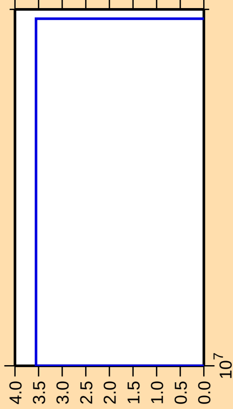
\Delta\sigma/\sigma vs. E for ^{194}\text{W}(\text{n},\text{nd})
