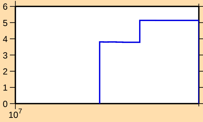
\Delta\sigma/\sigma vs. E for ^{112}\text{Xe}(n,\text{tot.})
