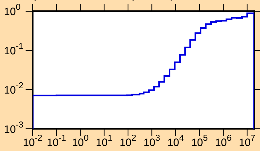
\mu vs. E for ^{112}\text{Xe}(\text{mt251})
