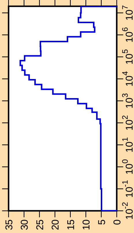
\Delta\mu/\mu vs. E for ^{112}\text{Xe}(\text{mt251})
