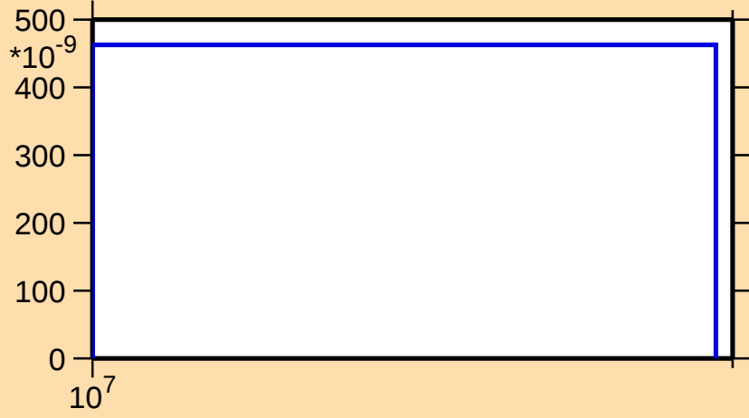
\sigma vs. E for ^{112}\text{Xe}(n,2n\alpha)
