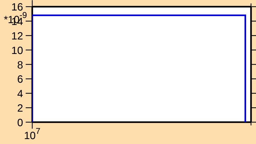
\sigma vs. E for ^{112}\text{Xe}(n,2np)
