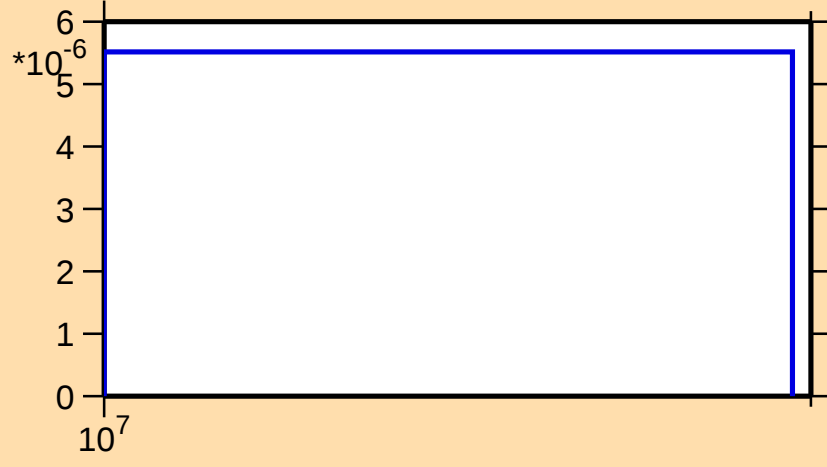
\sigma vs. E for ^{112}\text{Xe}(n,2n)
