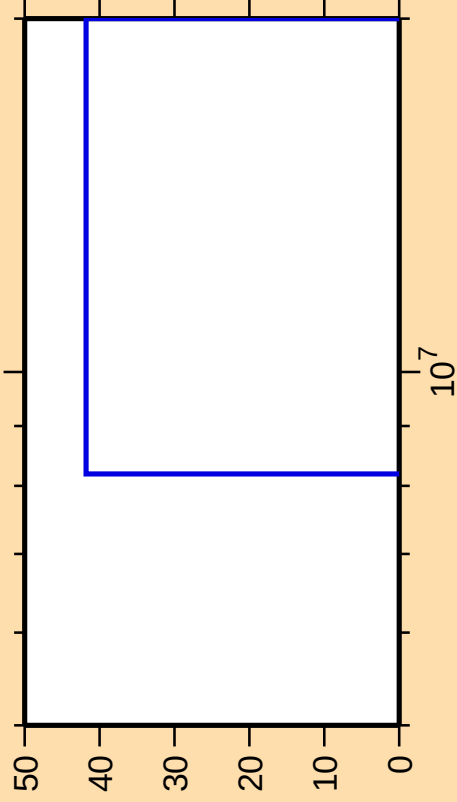
\Delta\sigma/\sigma vs. E for ^{112}\text{Xe}(n,n_1)
