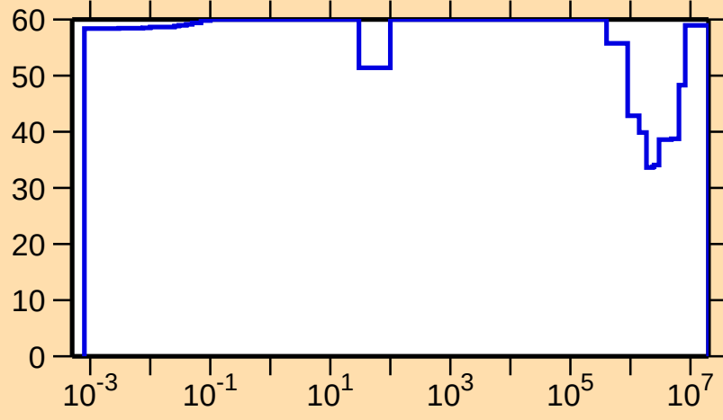
\Delta\sigma/\sigma vs. E for ^{112}\text{Xe}(n,\gamma)
