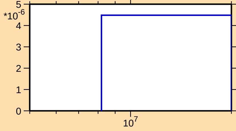
\sigma vs. E for ^{112}\text{Xe}(n,2n)
