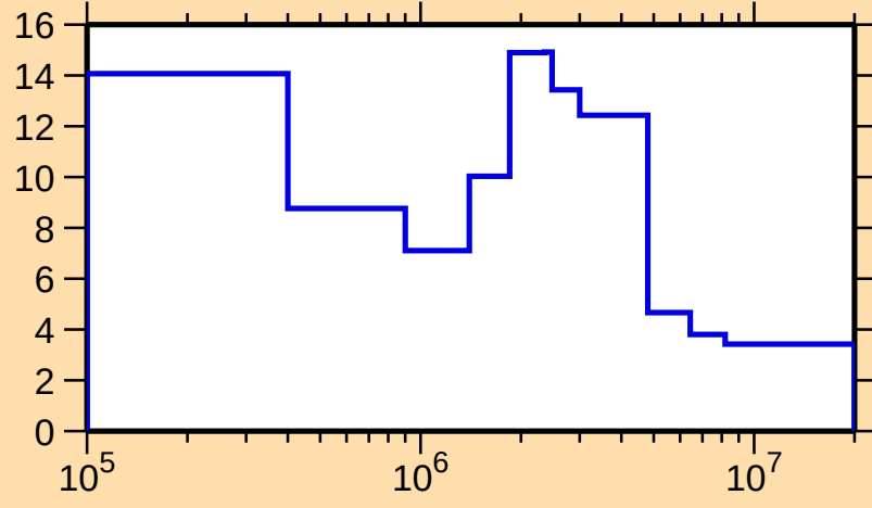
\Delta\sigma/\sigma vs. E for ^{112}\text{Xe}(n,\text{tot.})
