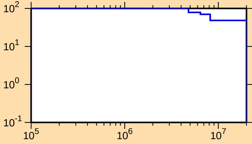
\Delta\sigma/\sigma vs. E for ^{112}\text{Xe}(n,n\text{cont.})
