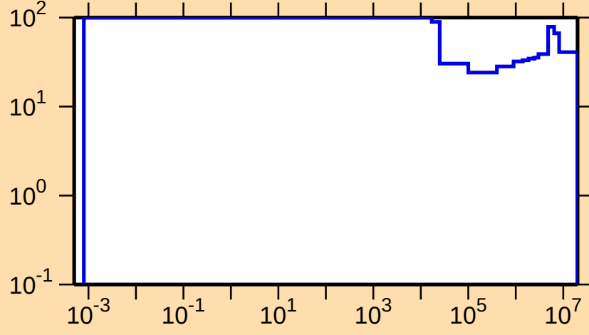
\Delta\sigma/\sigma vs. E for ^{112}\text{Xe}(n,p)
