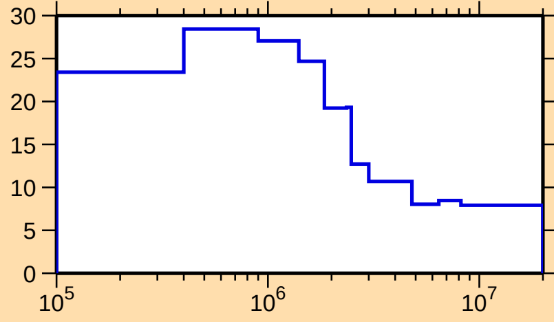
\Delta\sigma/\sigma vs. E for ^{112}\text{Xe}(n,n\text{onel.})
