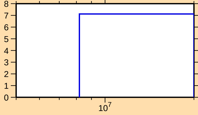
\Delta\sigma/\sigma vs. E for ^{112}\text{Xe}(n,\text{el.})
