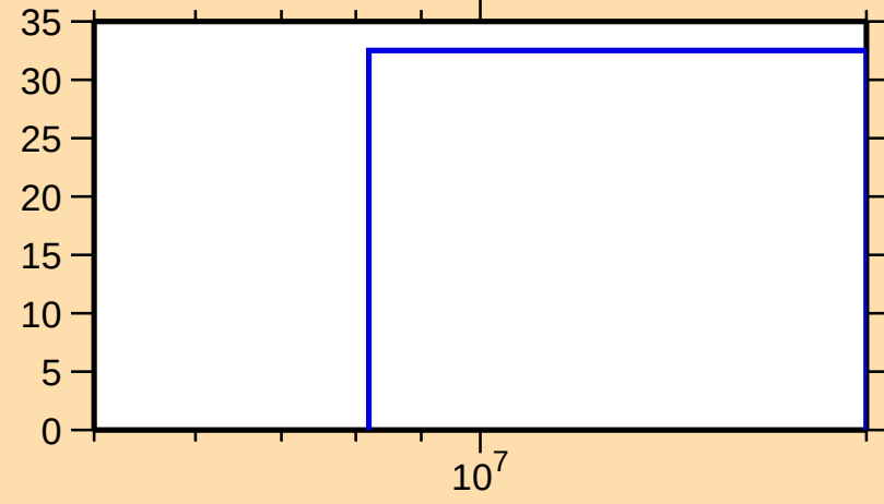
\Delta\sigma/\sigma vs. E for ^{112}\text{Xe}(n,\text{inel.})
