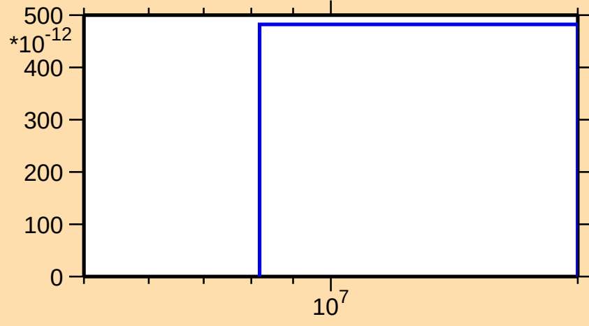
\sigma vs. E for ^{112}\text{Xe}(\text{mt } 34)
