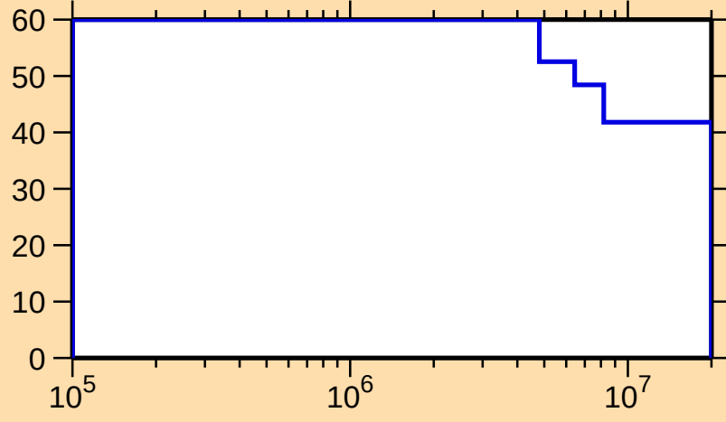
\Delta\sigma/\sigma vs. E for ^{112}\text{Xe}(n,n_1)
