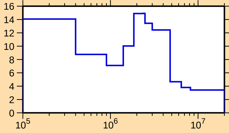
\Delta\sigma/\sigma vs. E for ^{112}\text{Xe}(n,\text{tot.})
