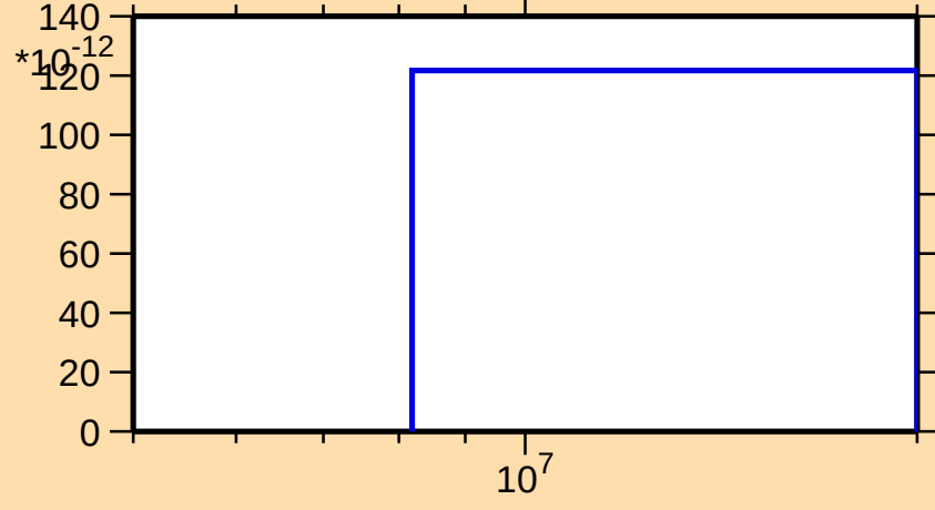
\sigma vs. E for ^{112}\text{Xe}(n,\text{nd})
