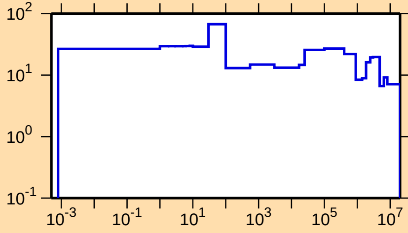
\Delta\sigma/\sigma vs. E for ^{112}\text{Xe}(n,\text{el.})
