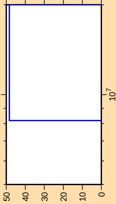
\Delta\sigma/\sigma vs. E for ^{112}\text{Xe}(n,n\text{cont.})
