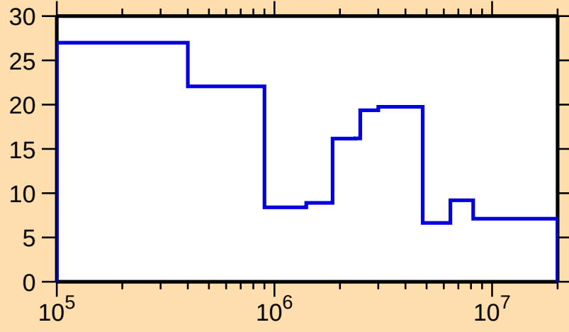
\Delta\sigma/\sigma vs. E for ^{112}\text{Xe}(n,\text{el.})
