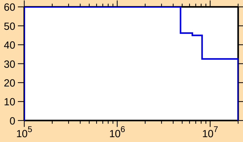
\Delta\sigma/\sigma vs. E for ^{112}\text{Xe}(n,\text{inel.})
