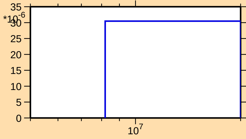
\sigma vs. E for ^{112}\text{Xe}(n,\text{pt})
