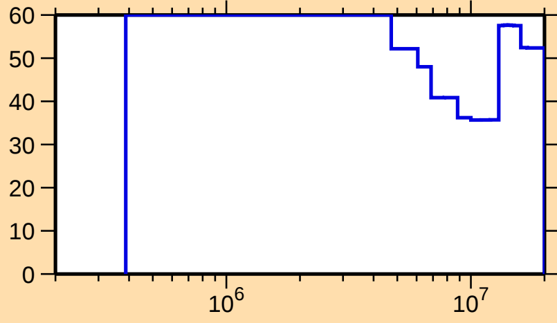
\Delta\sigma/\sigma vs. E for ^{116}\text{Xe}(n,n_1)
