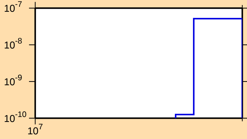
\sigma vs. E for ^{116}\text{Xe}(n,\text{nd})
