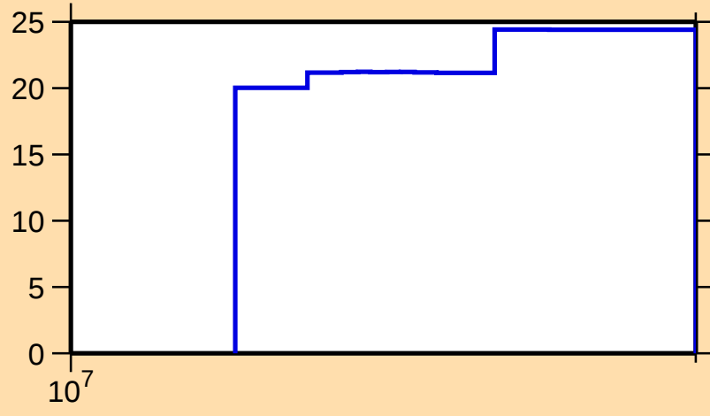
\Delta\sigma/\sigma vs. E for ^{116}\text{Xe}(n,\text{nonel.})
