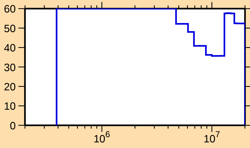
\Delta\sigma/\sigma vs. E for ^{116}\text{Xe}(n,n_1)
