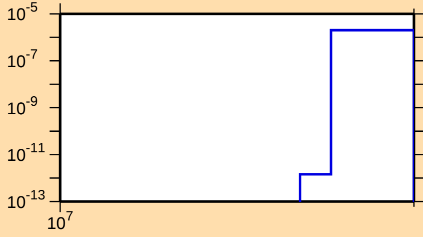
\sigma vs. E for ^{116}\text{Xe}(n,2np)
