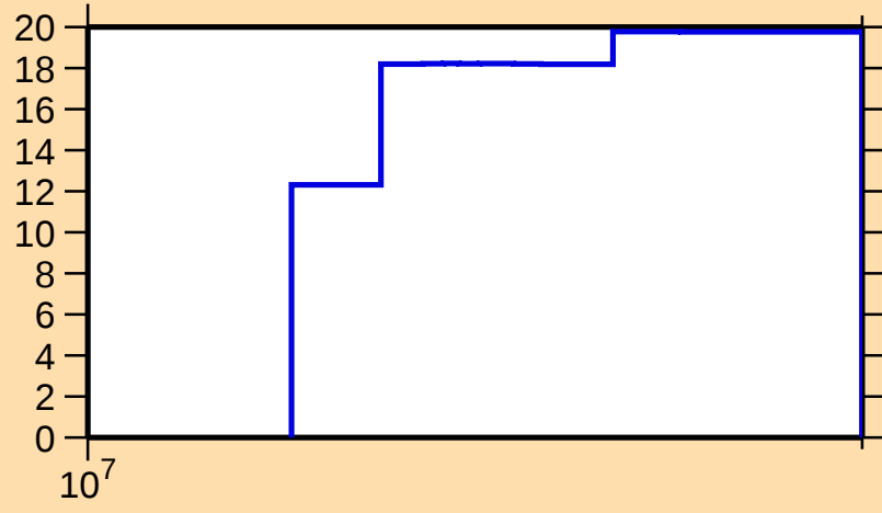
\Delta\sigma/\sigma vs. E for ^{116}\text{Xe}(n,\text{tot.})
