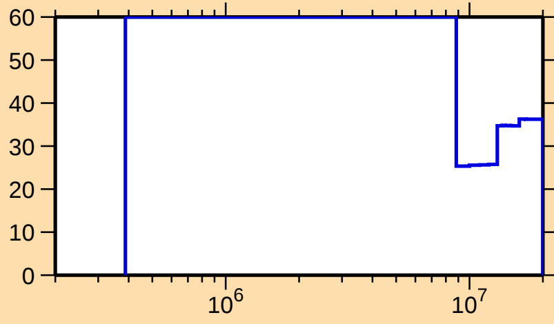
\Delta\sigma/\sigma vs. E for ^{116}\text{Xe}(n,\text{inel.})
