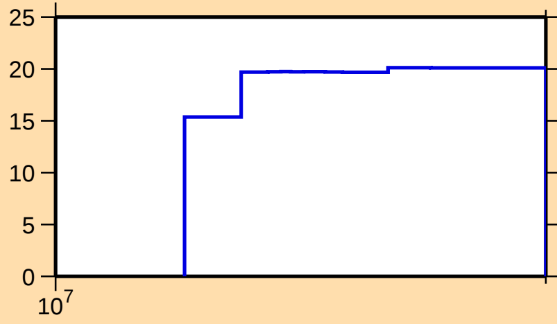
\Delta\sigma/\sigma vs. E for ^{116}\text{Xe}(n,\text{el.})
