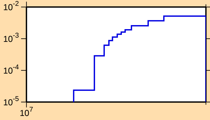
\sigma vs. E for ^{116}\text{Xe}(n,2n)
