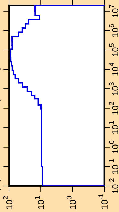
\Delta\mu/\mu vs. E for ^{116}\text{Xe}(\text{mt251})
