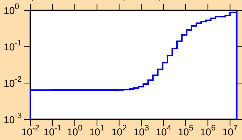
\mu vs. E for ^{116}\text{Xe}(\text{mt251})
