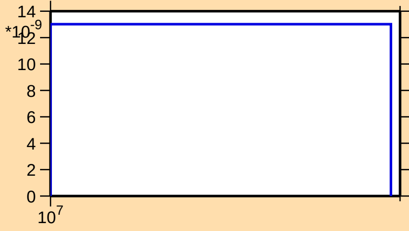
\sigma vs. E for ^{116}\text{Xe}(n,2np)
