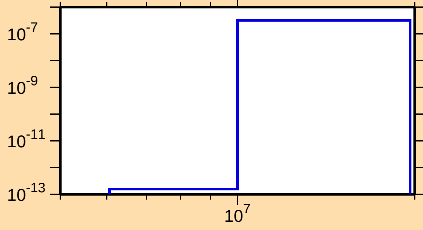
\sigma vs. E for ^{116}\text{Xe}(\text{mt117})
