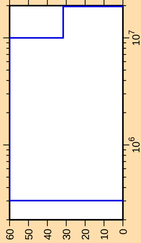
\Delta\sigma/\sigma vs. E for ^{116}\text{Xe}(n,\text{inel.})
