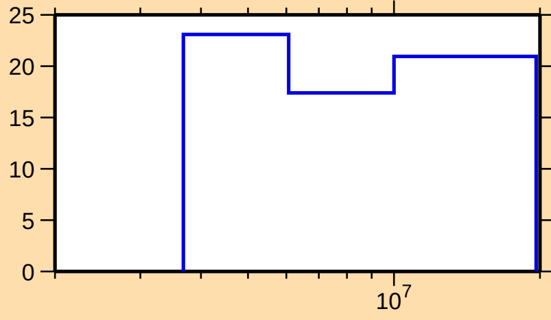
\Delta\sigma/\sigma vs. E for ^{116}\text{Xe}(n,n\text{onel.})
