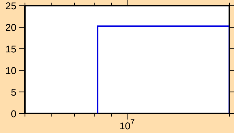
\Delta\sigma/\sigma vs. E for ^{116}\text{Xe}(n,\text{nonel.})
