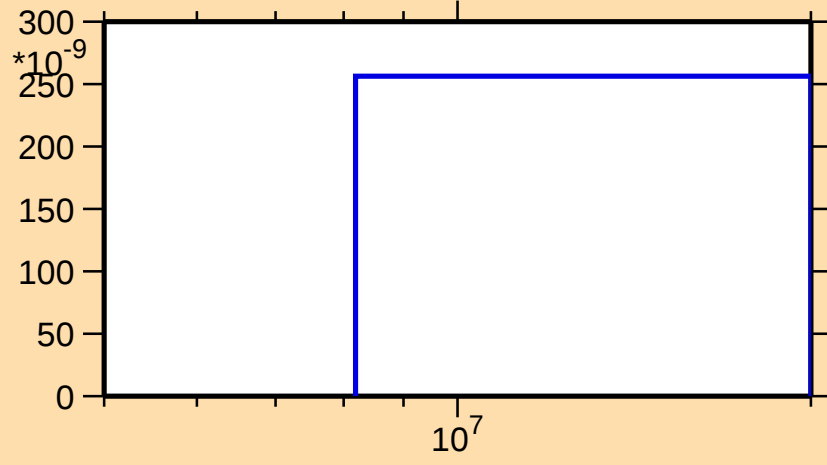
\sigma vs. E for ^{116}\text{Xe}(\text{mt117})
