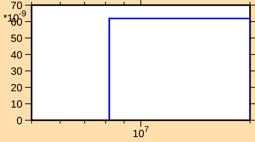
\sigma vs. E for ^{116}\text{Xe}(n,\text{pt})
