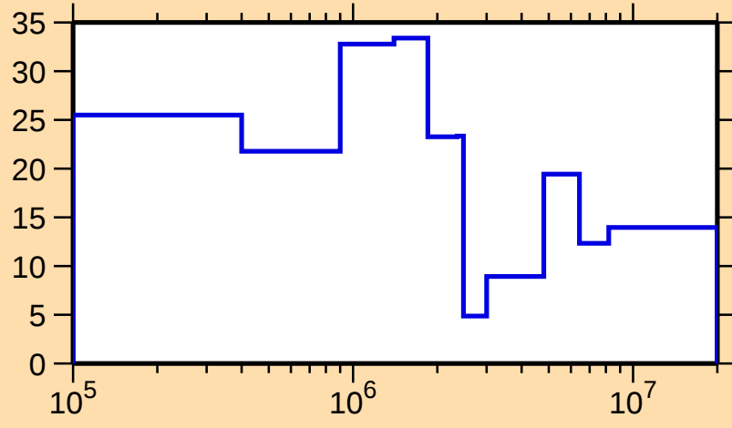
\Delta\sigma/\sigma vs. E for ^{116}\text{Xe}(n,\text{tot.})
