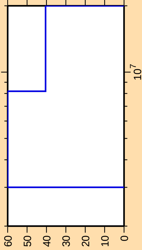
\Delta\sigma/\sigma vs. E for ^{116}\text{Xe}(n,\text{ncont.})
