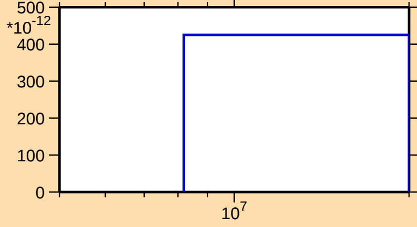
\sigma vs. E for ^{116}\text{Xe}(n,\text{nd})
