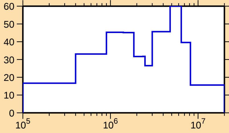
\Delta\sigma/\sigma vs. E for ^{116}\text{Xe}(n,\text{el.})
