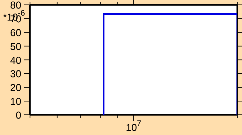
\sigma vs. E for ^{116}\text{Xe}(n,t)
