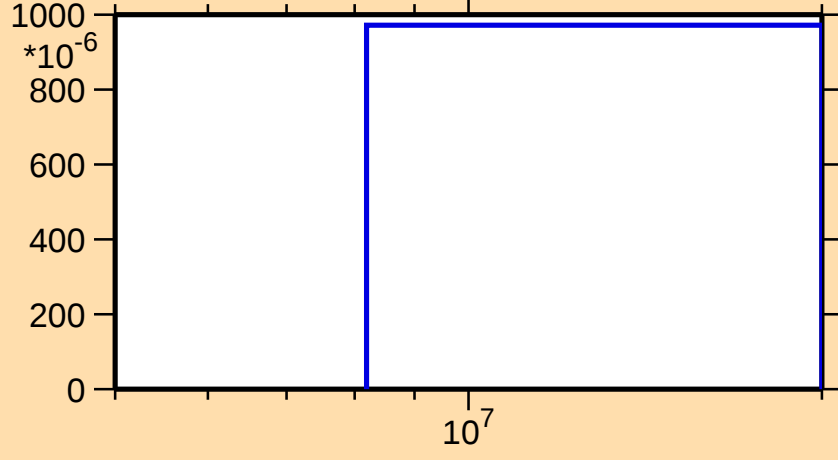
\sigma vs. E for ^{116}\text{Xe}(n,2n)
