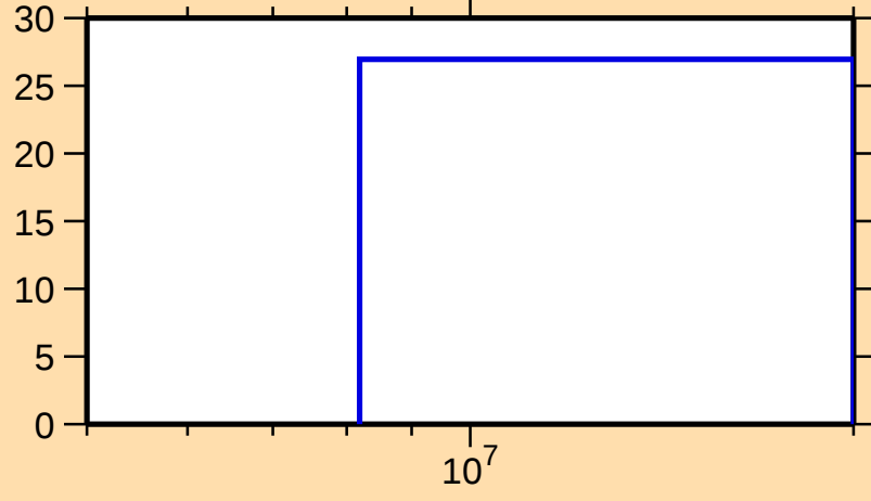
\Delta\sigma/\sigma vs. E for ^{116}\text{Xe}(n,\text{inel.})
