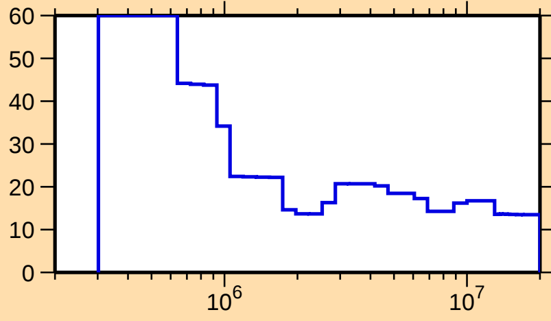
\Delta\sigma/\sigma vs. E for ^{118}\text{Xe}(n,\text{nonel.})
