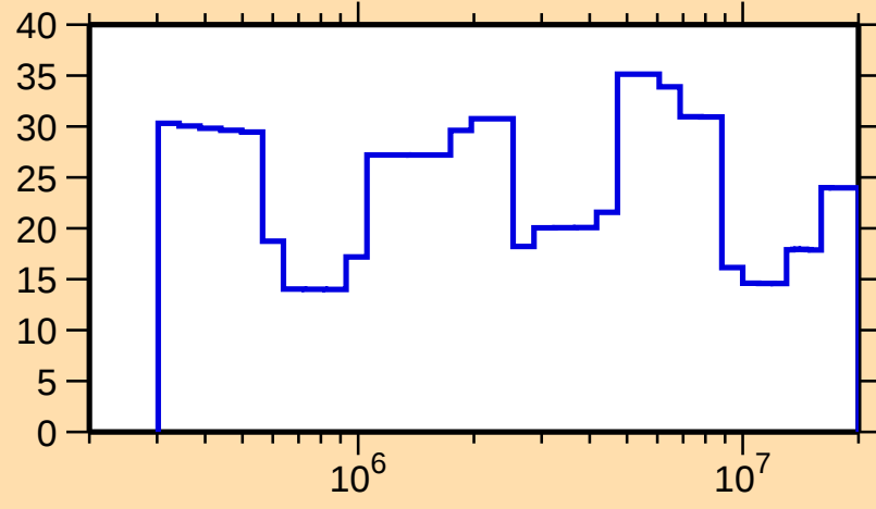
\Delta\sigma/\sigma vs. E for ^{118}\text{Xe}(n,\text{el.})
