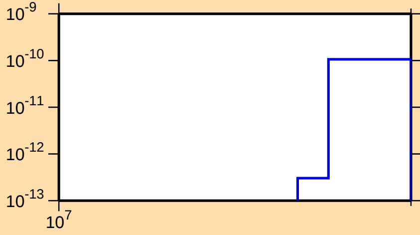
\sigma vs. E for ^{118}\text{Xe}(\text{mt } 34)
