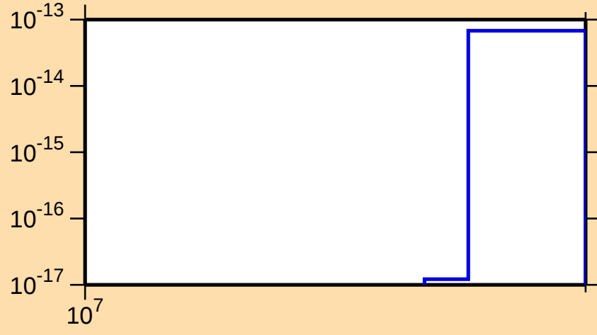
\sigma vs. E for ^{118}\text{Xe}(n,nt)
