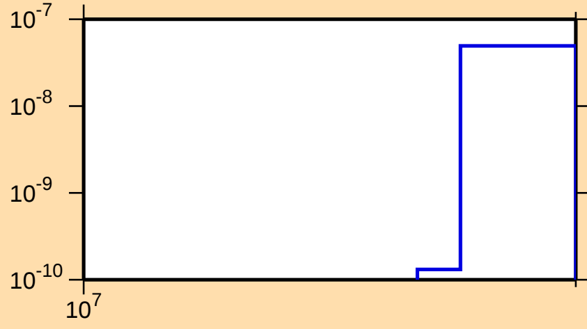
\sigma vs. E for ^{118}\text{Xe}(n,\text{pt})
