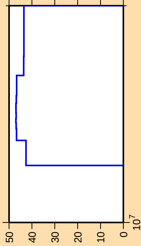
\Delta\sigma/\sigma vs. E for ^{118}\text{Xe}(n,n_1)
