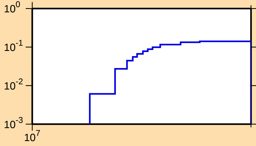
\sigma vs. E for ^{118}\text{Xe}(n,2n)
