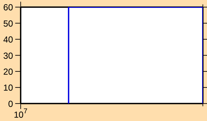
\Delta\sigma/\sigma vs. E for ^{118}\text{Xe}(n,\text{inel.})
