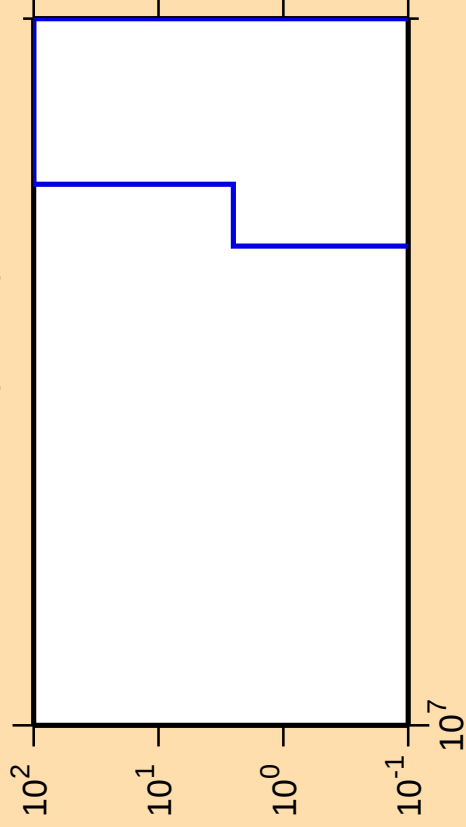
\Delta\sigma/\sigma vs. E for ^{118}\text{Xe}(\text{mt } 34)
