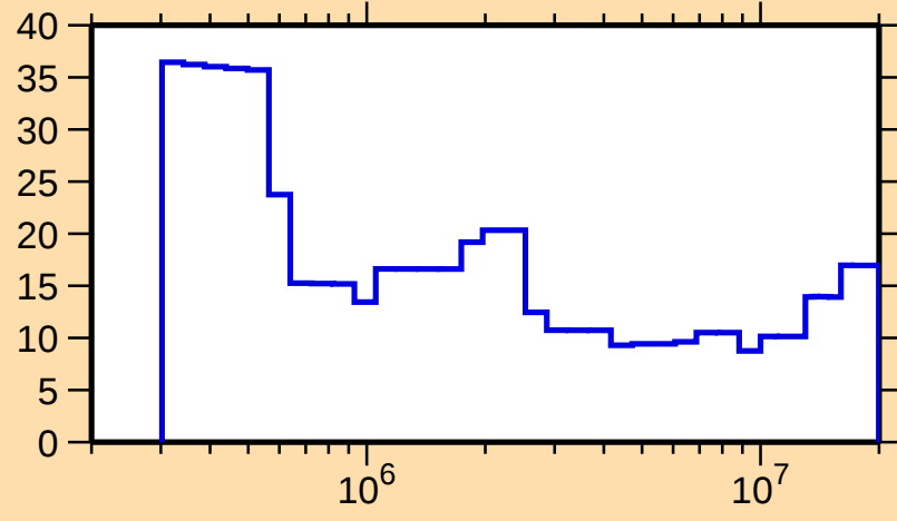
\Delta\sigma/\sigma vs. E for ^{118}\text{Xe}(n,\text{tot.})
