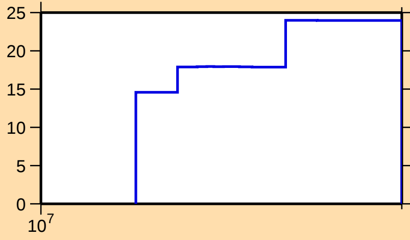
\Delta\sigma/\sigma vs. E for ^{118}\text{Xe}(n,\text{el.})
