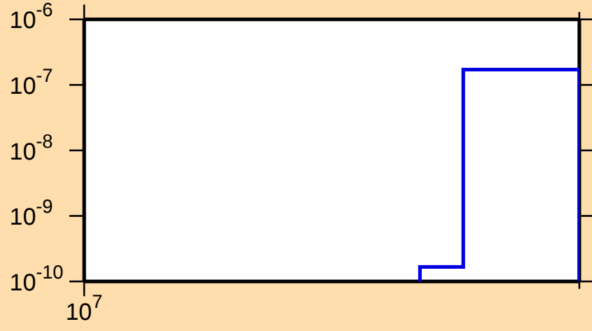
\sigma vs. E for ^{118}\text{Xe}(n,\text{nd})
