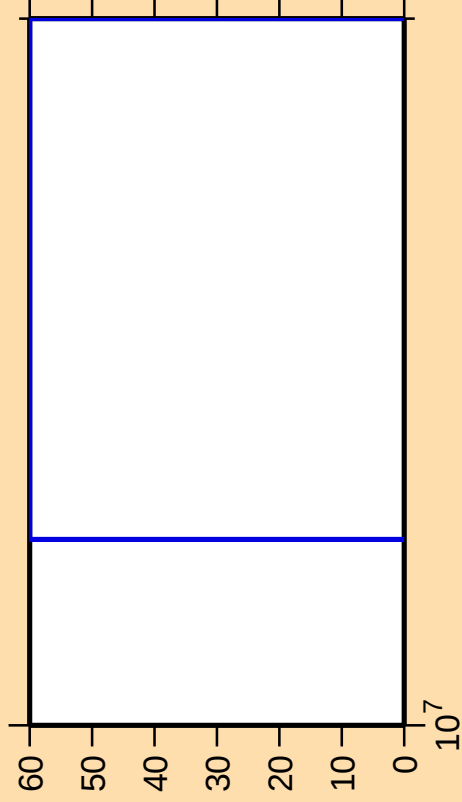
\Delta\sigma/\sigma vs. E for ^{118}\text{Xe}(n,\gamma)
