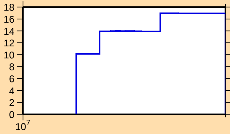
\Delta\sigma/\sigma vs. E for ^{118}\text{Xe}(n,\text{tot.})
