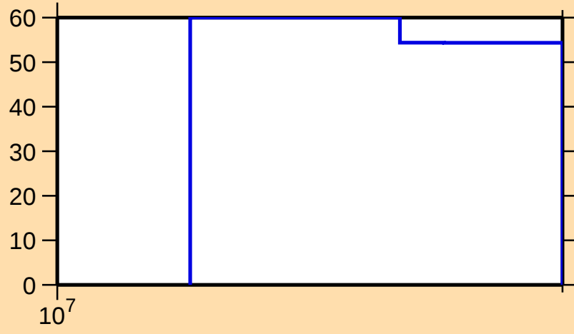
\Delta\sigma/\sigma vs. E for ^{118}\text{Xe}(n,2n)
