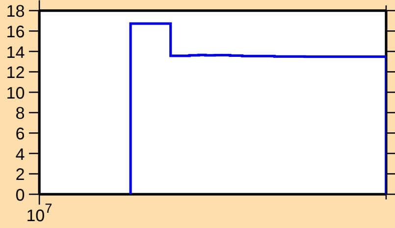
\Delta\sigma/\sigma vs. E for ^{118}\text{Xe}(n,\text{nonel.})
