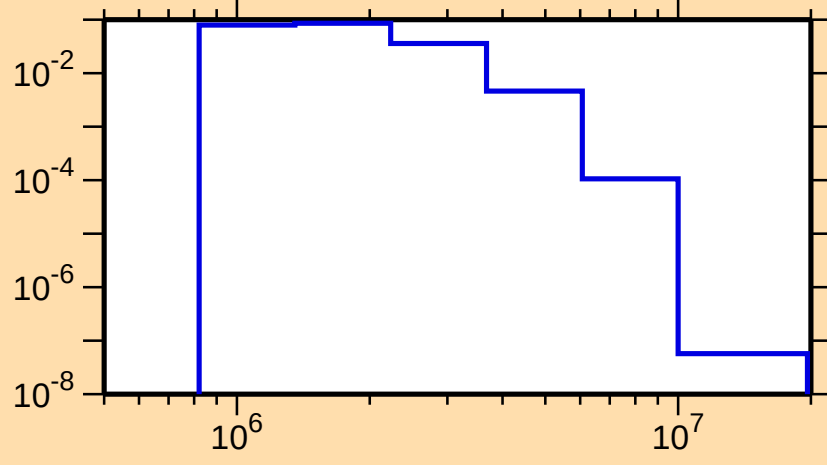
\sigma vs. E for ^{118}\text{Xe}(n,n_3)
