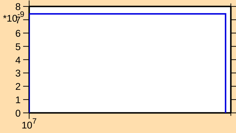
\sigma vs. E for ^{118}\text{Xe}(n,2np)
