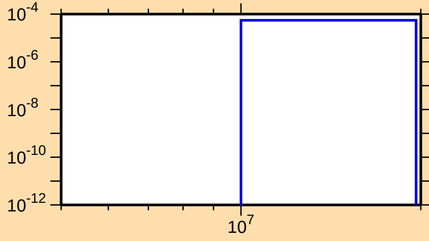
\sigma vs. E for ^{118}\text{Xe}(n,t)
