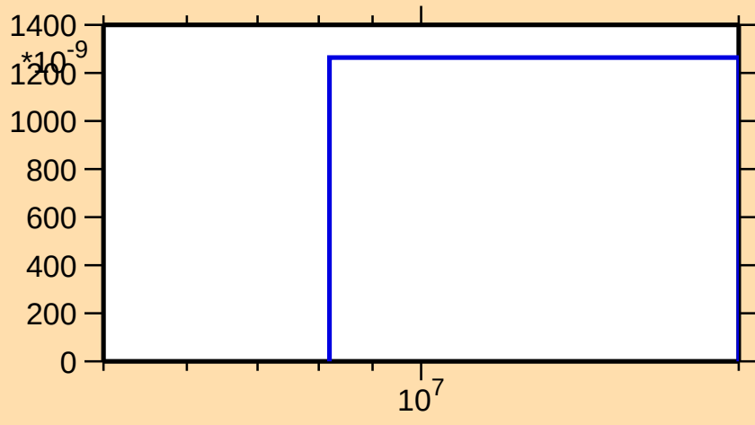
\sigma vs. E for ^{118}\text{Xe}(\text{mt } 45)
