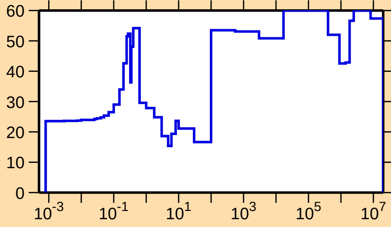
\Delta\sigma/\sigma vs. E for ^{118}\text{Xe}(n,\gamma)
