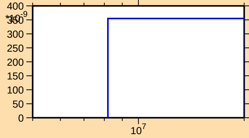
\sigma vs. E for ^{119}\text{Xe}(n,\text{nd})
