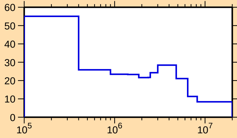
\Delta\sigma/\sigma vs. E for ^{119}\text{Xe}(n,\text{tot.})
