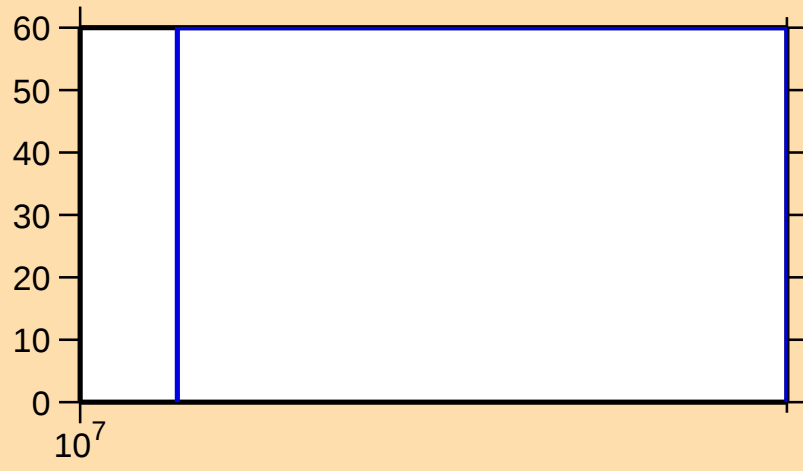
\Delta\sigma/\sigma vs. E for ^{120}\text{Xe}(n,2n)
