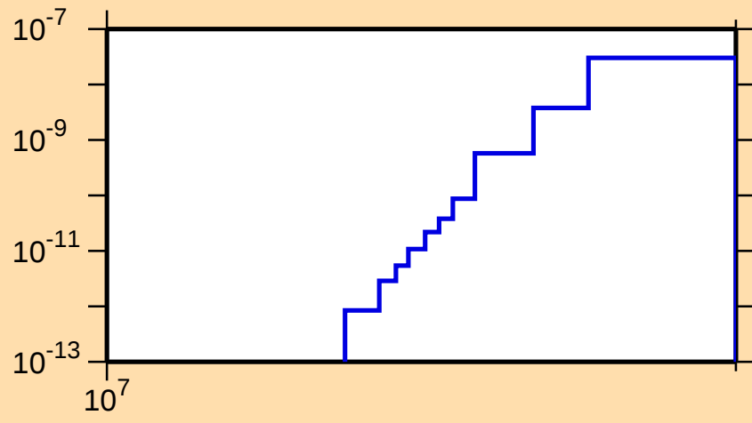
\sigma vs. E for ^{120}\text{Xe}(\text{mt117})
