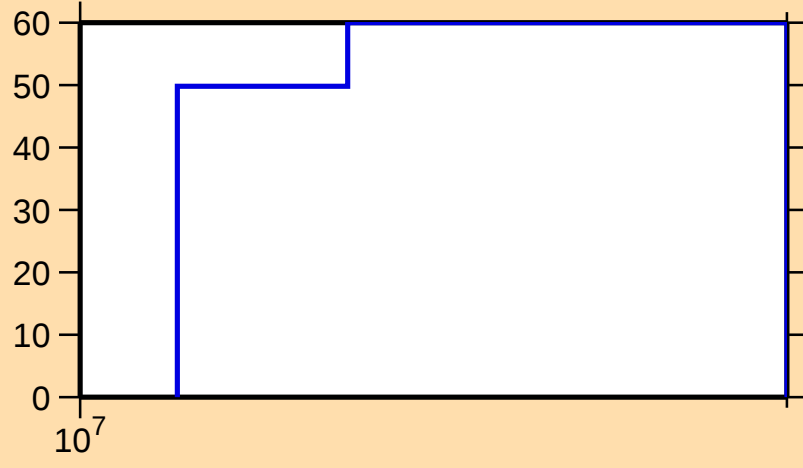
\Delta\sigma/\sigma vs. E for ^{120}\text{Xe}(n,\text{inel.})
