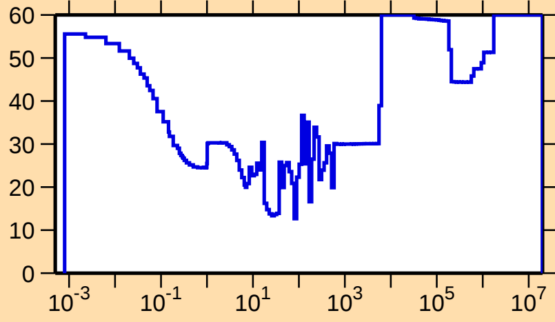
\Delta\sigma/\sigma vs. E for ^{120}\text{Xe}(n,\gamma)
