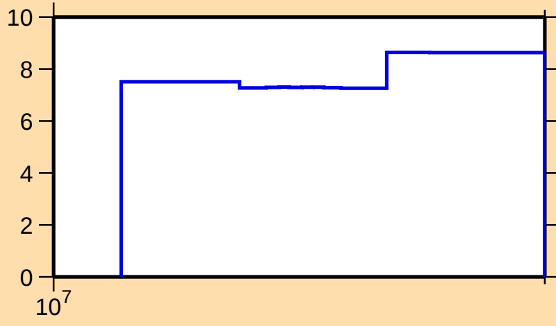
\Delta\sigma/\sigma vs. E for ^{120}\text{Xe}(n,\text{nonel.})
