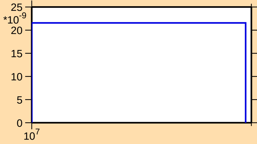
\sigma vs. E for ^{120}\text{Xe}(\text{mt } 45)
