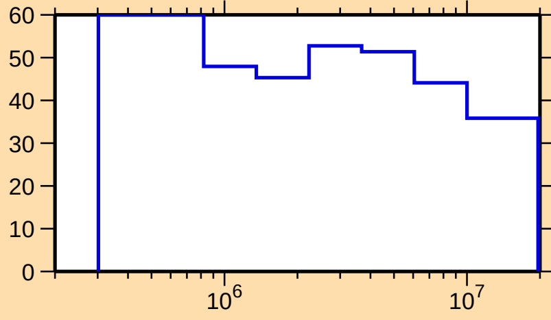
\Delta\sigma/\sigma vs. E for ^{120}\text{Xe}(n,n_1)
