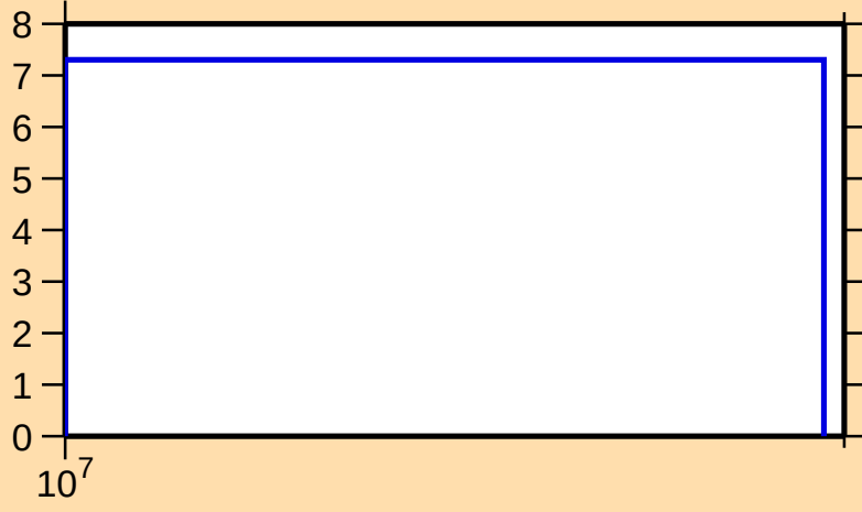
\Delta\sigma/\sigma vs. E for ^{120}\text{Xe}(n,\text{nonel.})
