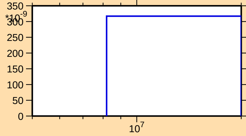
\sigma vs. E for ^{120}\text{Xe}(n,\text{pd})
