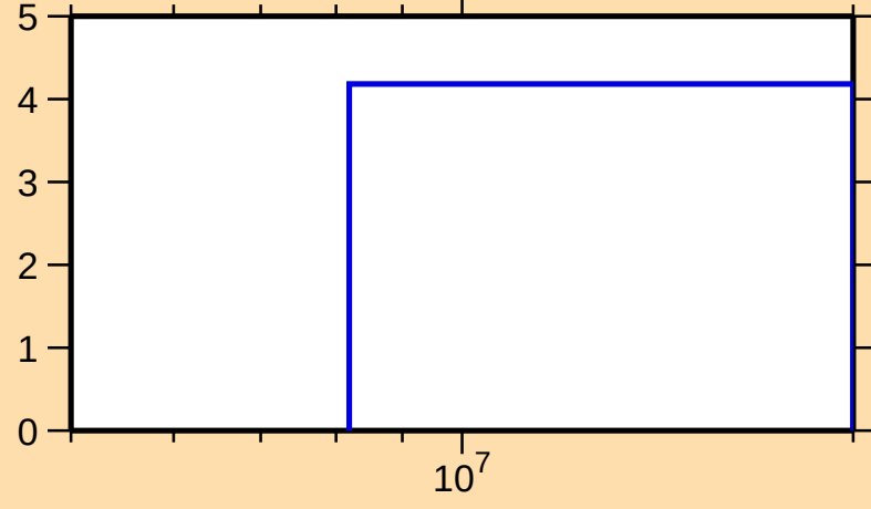
\Delta\sigma/\sigma vs. E for ^{120}\text{Xe}(n,\text{tot.})
