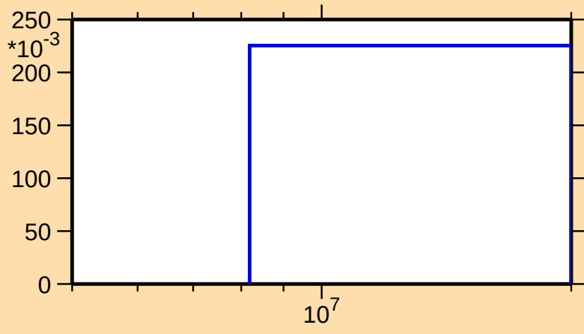
\sigma vs. E for ^{120}\text{Xe}(n,2n)
