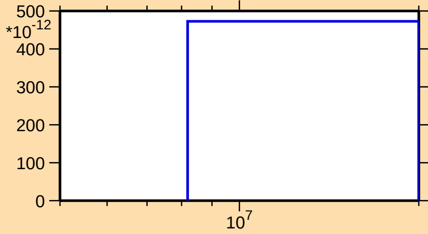
\sigma vs. E for ^{120}\text{Xe}(\text{mt117})
