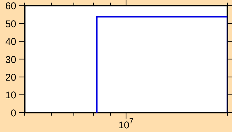
\Delta\sigma/\sigma vs. E for ^{120}\text{Xe}(n,\text{inel.})
