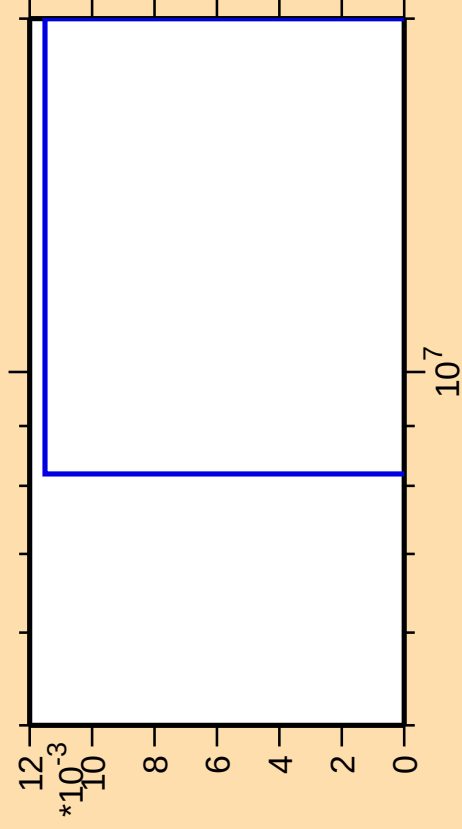
\Delta\sigma/\sigma vs. E for ^{120}\text{Xe}(n,nt)
