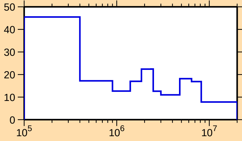
\Delta\sigma/\sigma vs. E for ^{120}\text{Xe}(n,\text{el.})
