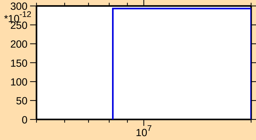
\sigma vs. E for ^{120}\text{Xe}(n,\text{nd})
