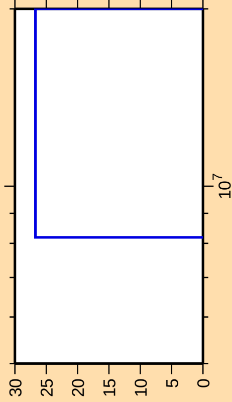
\Delta\sigma/\sigma vs. E for ^{120}\text{Xe}(n,\text{pt})
