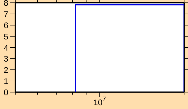
\Delta\sigma/\sigma vs. E for ^{120}\text{Xe}(n,\text{el.})
