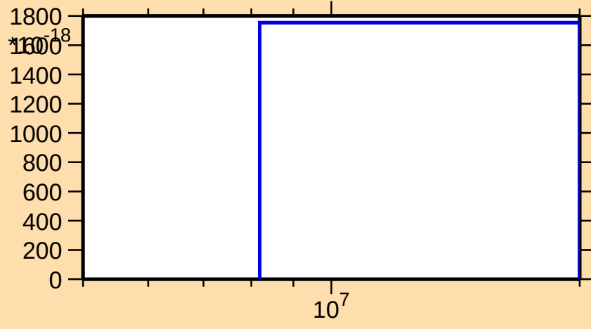
\sigma vs. E for ^{120}\text{Xe}(n,nt)
