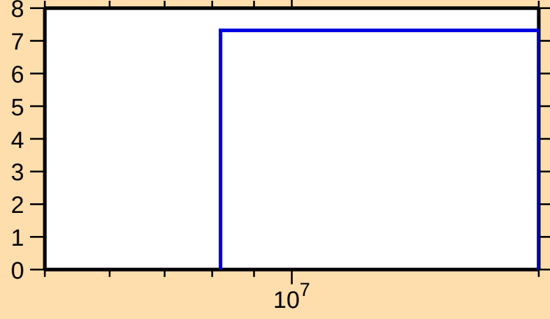
\Delta\sigma/\sigma vs. E for ^{120}\text{Xe}(n,\text{nonel.})
