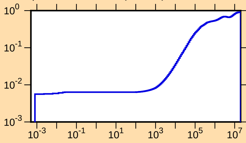
\mu vs. E for ^{121}\text{Xe}(\text{mt251})
