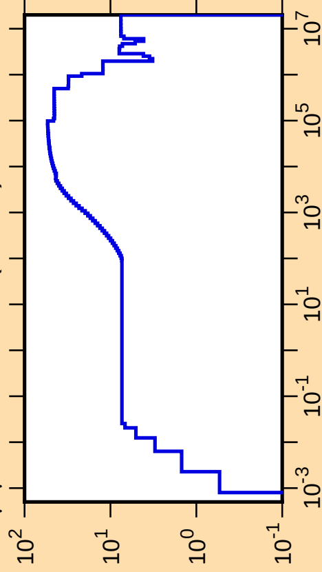
\Delta\mu/\mu vs. E for ^{121}\text{Xe}(\text{mt251})
