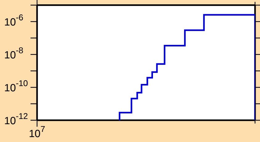
\sigma vs. E for ^{121}\text{Xe}(n,\text{pd})
