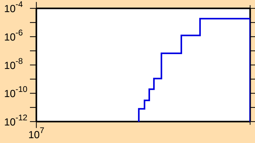
\sigma vs. E for ^{121}\text{Xe}(n,\text{nd})
