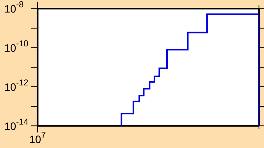
\sigma vs. E for ^{121}\text{Xe}(\text{mt117})
