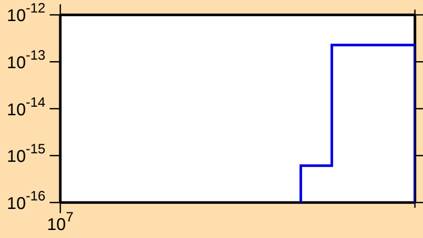
\sigma vs. E for ^{121}\text{Xe}(n,nt)
