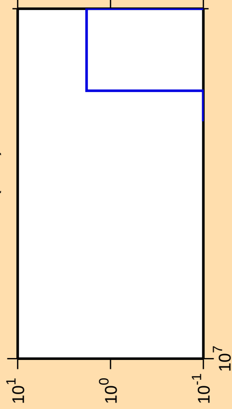
\Delta\sigma/\sigma vs. E for ^{121}\text{Xe}(n,nt)
