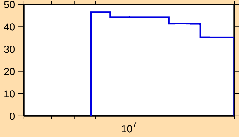
\Delta\sigma/\sigma vs. E for ^{121}\text{Xe}(n,2n)
