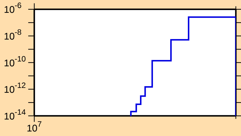
\sigma vs. E for ^{121}\text{Xe}(n,\text{pt})
