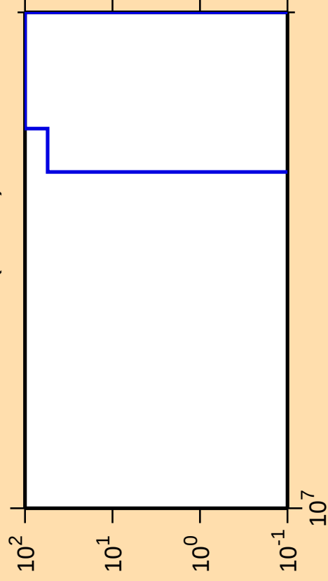
\Delta\sigma/\sigma vs. E for ^{121}\text{Xe}(\text{mt } 34)
