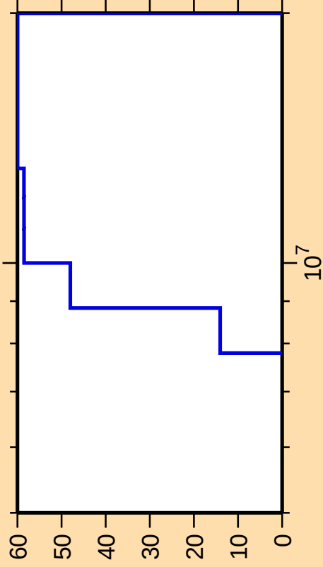
\Delta\sigma/\sigma vs. E for ^{121}\text{Xe}(n,n\text{cont.})
