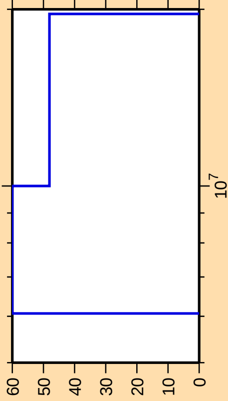
\Delta\sigma/\sigma vs. E for ^{121}\text{Xe}(n,p)
