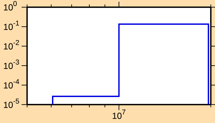
\sigma vs. E for ^{121}\text{Xe}(n,np)
