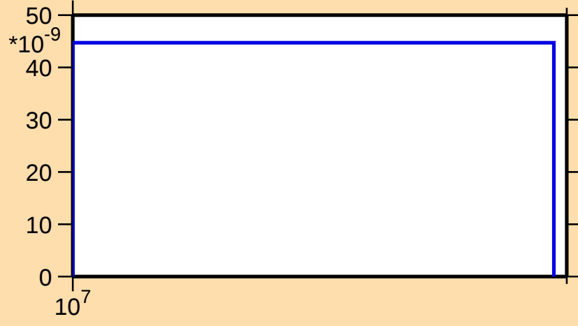
\sigma vs. E for ^{121}\text{Xe}(n,\text{pd})
