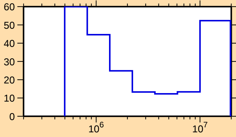
\Delta\sigma/\sigma vs. E for ^{121}\text{Xe}(n,\text{inel.})
