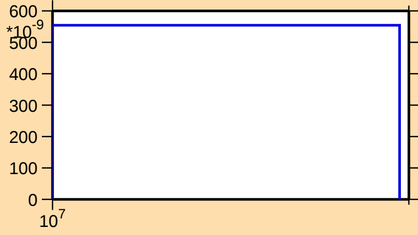
\sigma vs. E for ^{121}\text{Xe}(n,2n\alpha)
