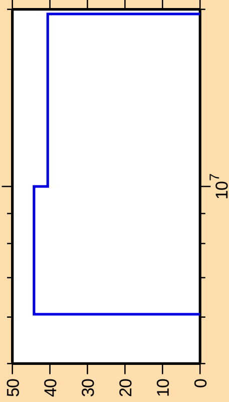
\Delta\sigma/\sigma vs. E for ^{121}\text{Xe}(n,2n)
