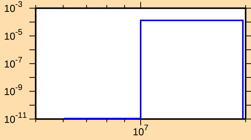
\sigma vs. E for ^{121}\text{Xe}(n,t)
