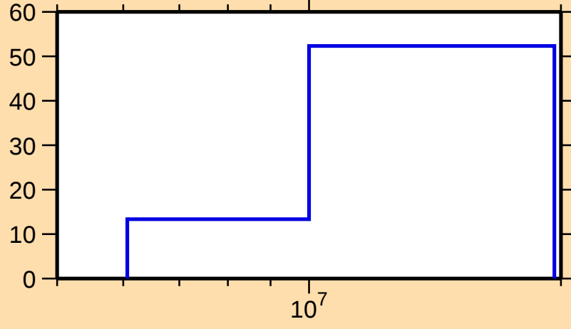
\Delta\sigma/\sigma vs. E for ^{121}\text{Xe}(n,\text{inel.})
