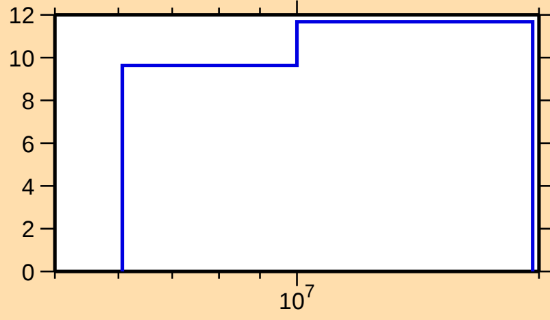
\Delta\sigma/\sigma vs. E for ^{121}\text{Xe}(n,\text{el.})
