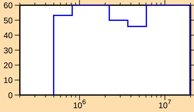
\Delta\sigma/\sigma vs. E for ^{121}\text{Xe}(n,n_1)
