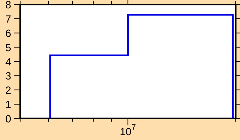
\Delta\sigma/\sigma vs. E for ^{121}\text{Xe}(n,\text{tot.})
