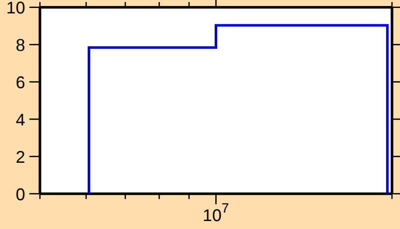
\Delta\sigma/\sigma vs. E for ^{121}\text{Xe}(n,\text{nonel.})
