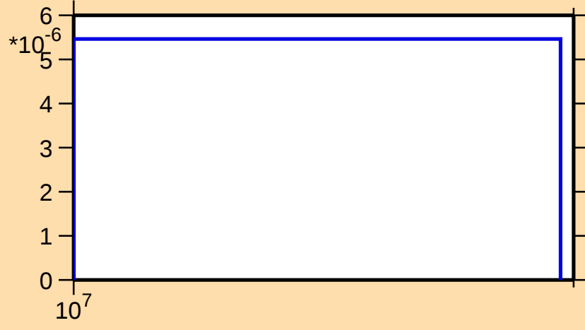
\sigma vs. E for ^{121}\text{Xe}(n,2np)
