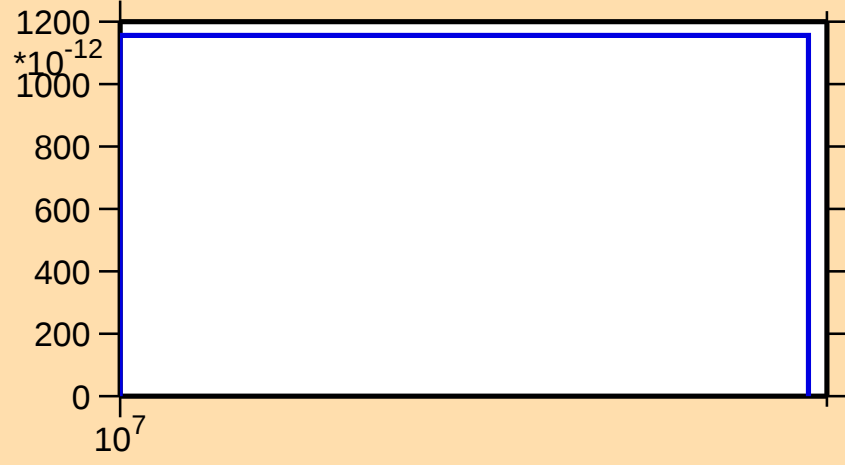
\sigma vs. E for ^{121}\text{Xe}(\text{mt } 45)
