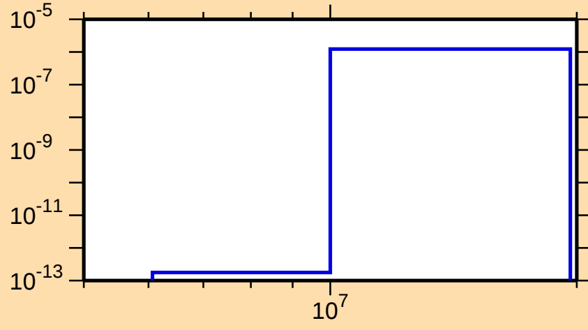
\sigma vs. E for ^{121}\text{Xe}(n,\text{He}3)
