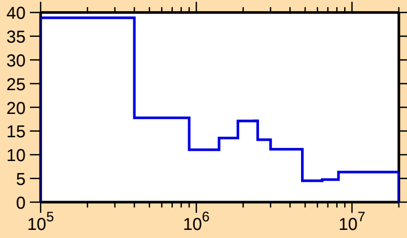
\Delta\sigma/\sigma vs. E for ^{121}\text{Xe}(n,\text{tot.})
