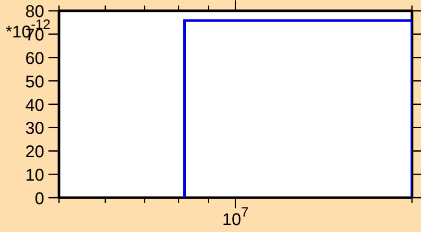
\sigma vs. E for ^{121}\text{Xe}(\text{mt117})
