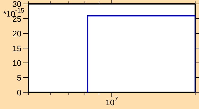
\sigma vs. E for ^{121}\text{Xe}(n,3n)
