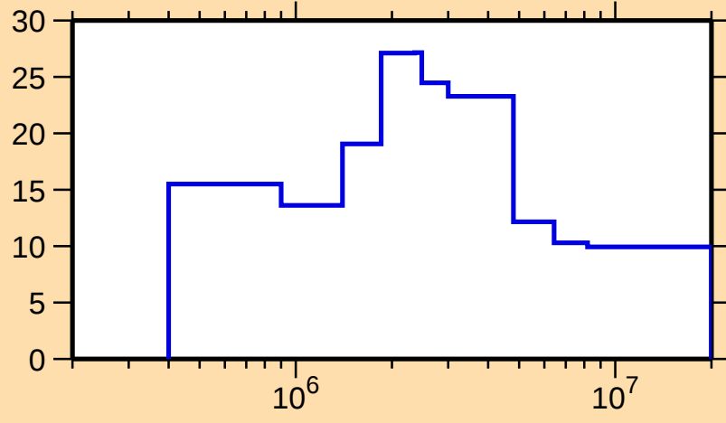
\Delta\sigma/\sigma vs. E for ^{121}\text{Xe}(n,\text{el.})
