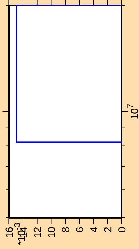
\Delta\sigma/\sigma vs. E for ^{121}\text{Xe}(n,nt)
