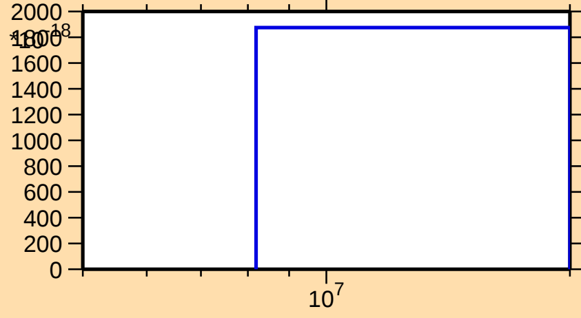
\sigma vs. E for ^{121}\text{Xe}(n,nt)
