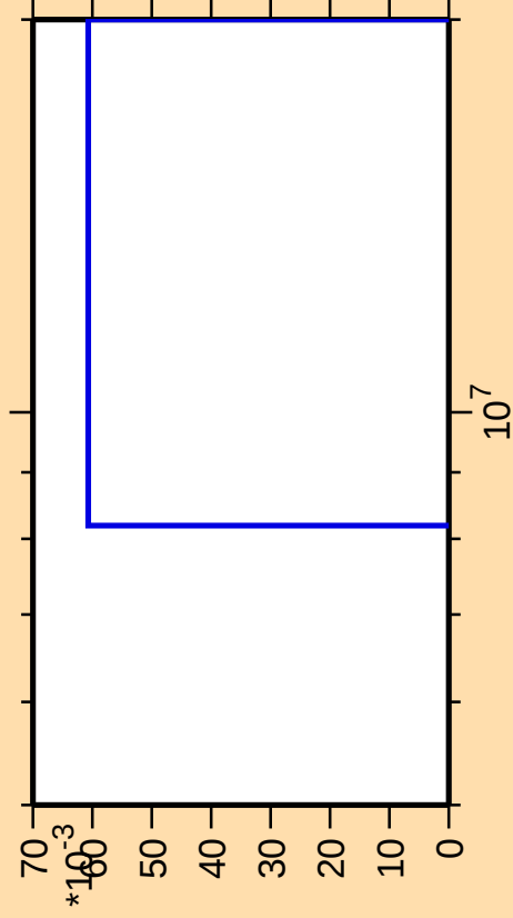
\Delta\sigma/\sigma vs. E for ^{121}\text{Xe}(n,3n)
