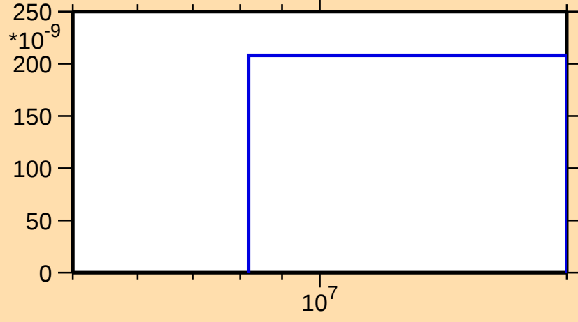
\sigma vs. E for ^{121}\text{Xe}(n,\text{nd})
