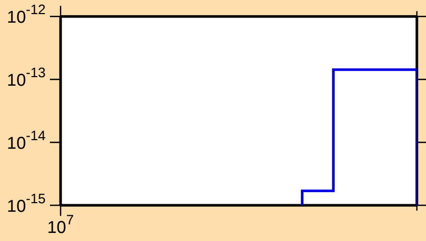
\sigma vs. E for ^{125}\text{Xe}(\text{mt117})
