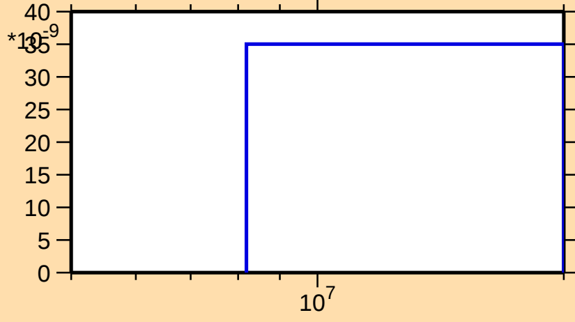
\sigma vs. E for ^{125}\text{Xe}(n,p\alpha)
