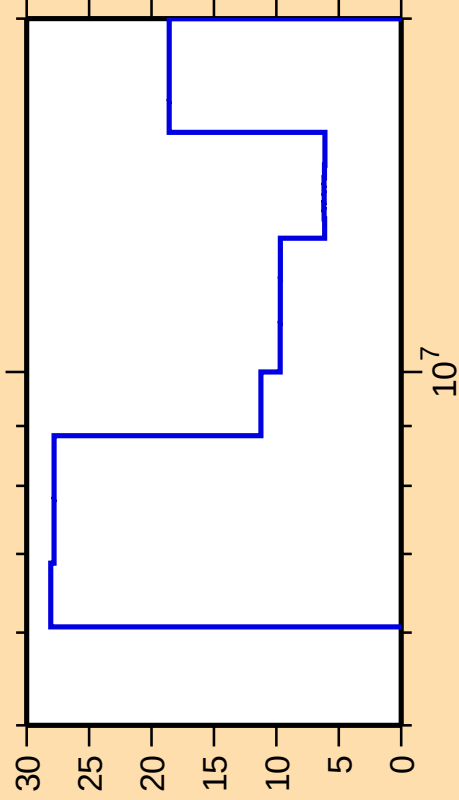
\Delta\sigma/\sigma vs. E for ^{131}\text{Xe}(n,2n)
