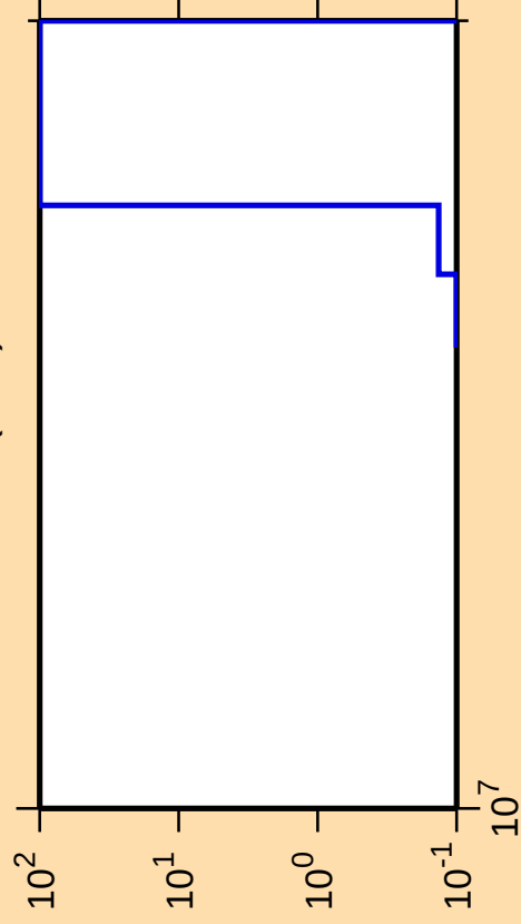
\Delta\sigma/\sigma vs. E for ^{131}\text{Xe}(n,\text{nt})
