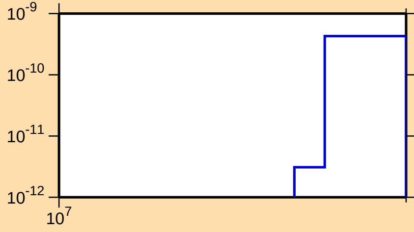
\sigma vs. E for ^{131}\text{Xe}(n,\text{He3})
