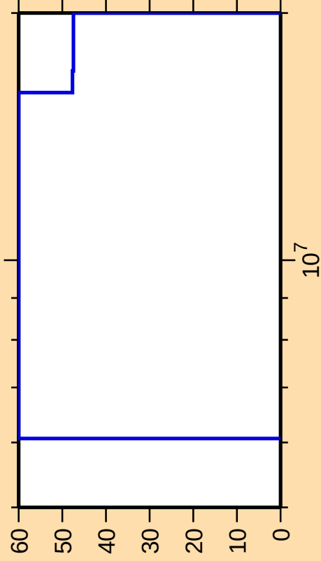
\Delta\sigma/\sigma vs. E for ^{131}\text{Xe}(n,\alpha)
