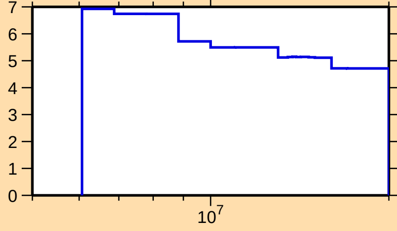
\Delta\sigma/\sigma vs. E for ^{131}\text{Xe}(n,\text{nonel.})
