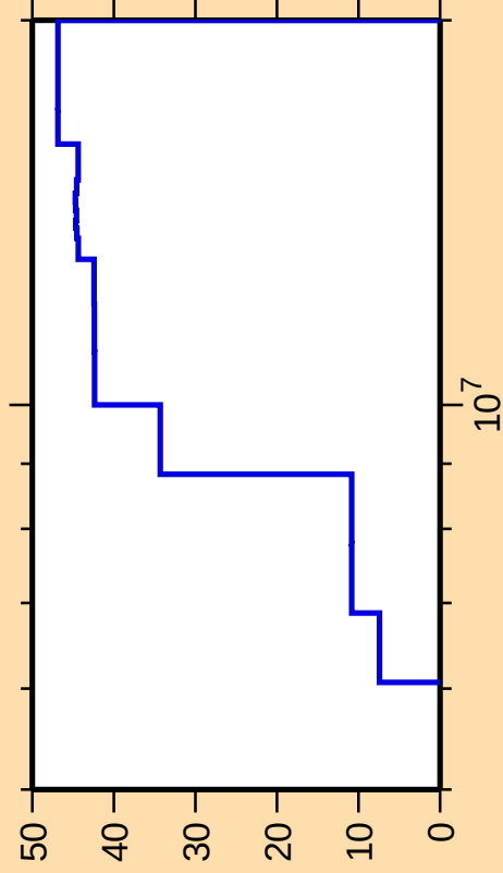
\Delta\sigma/\sigma vs. E for ^{131}\text{Xe}(n,n\text{cont.})
