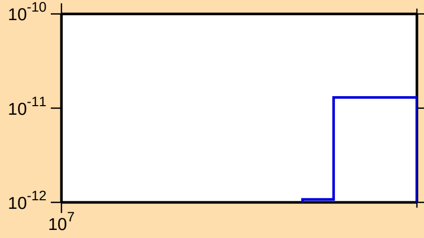
\sigma vs. E for ^{131}\text{Xe}(n,p\alpha)
