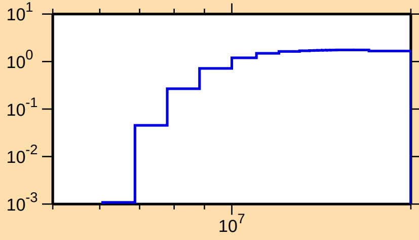
\sigma vs. E for ^{131}\text{Xe}(n,2n)
