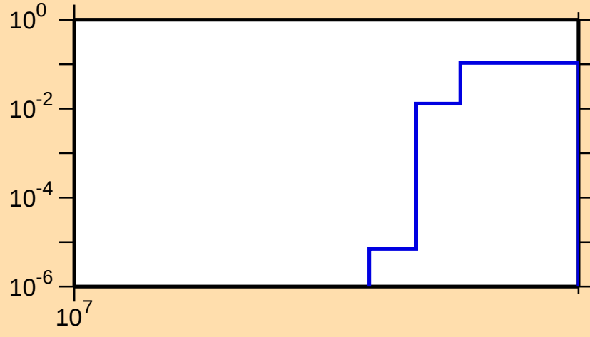
\sigma vs. E for ^{131}\text{Xe}(n,3n)
