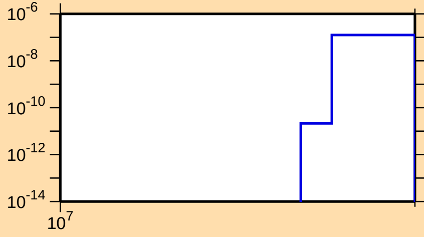
\sigma vs. E for ^{131}\text{Xe}(n,2np)
