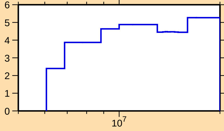
\Delta\sigma/\sigma vs. E for ^{131}\text{Xe}(n,\text{tot.})
