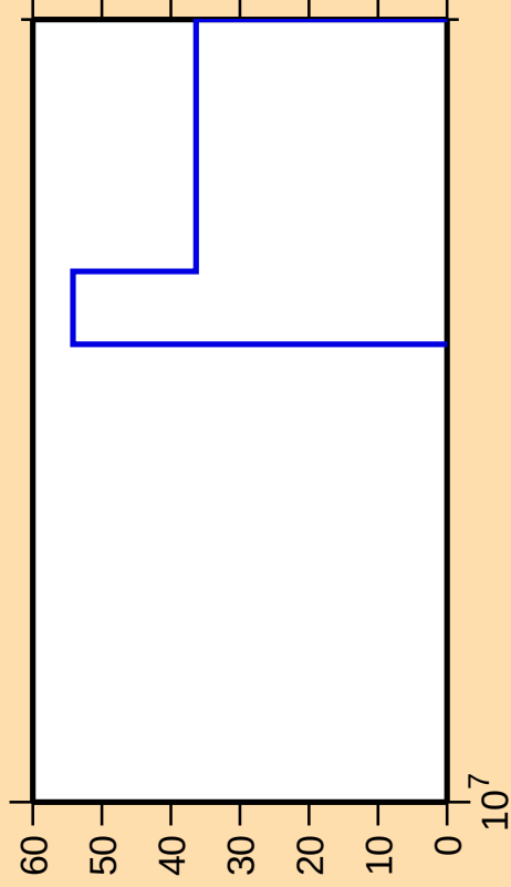
\Delta\sigma/\sigma vs. E for ^{131}\text{Xe}(n,3n)
