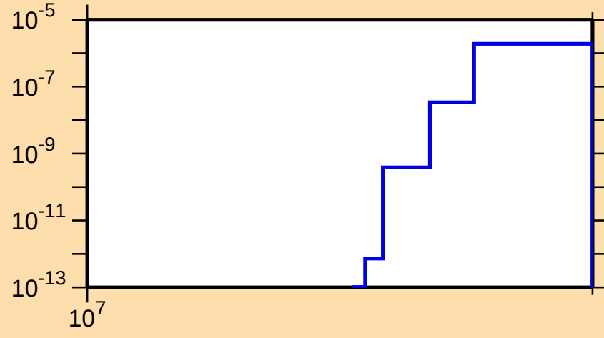
\sigma vs. E for ^{131}\text{Xe}(n,\text{nd})
