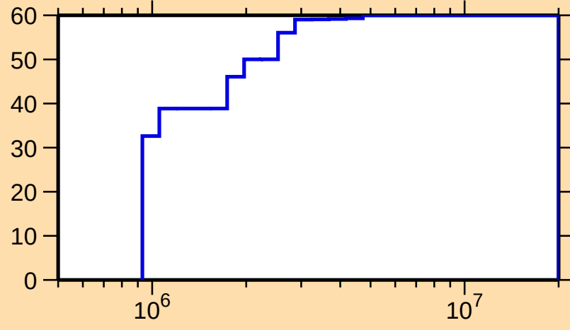
\Delta\sigma/\sigma vs. E for ^{131}\text{Xe}(n,\gamma)
