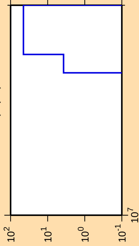
\Delta\sigma/\sigma vs. E for ^{131}\text{Xe}(n,p\alpha)
