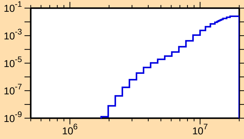
\sigma vs. E for ^{131}\text{Xe}(n,p)
