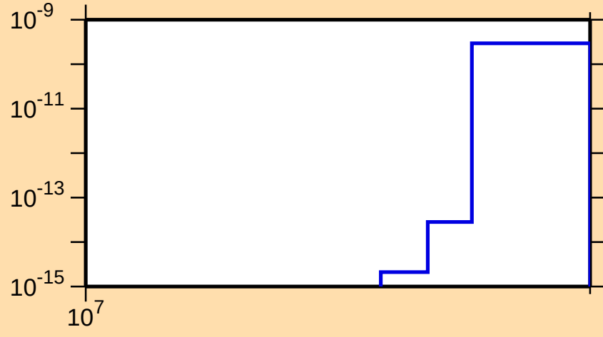
\sigma vs. E for ^{131}\text{Xe}(n,\text{nt})
