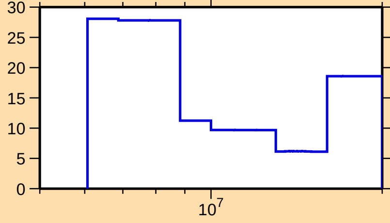
\Delta\sigma/\sigma vs. E for ^{131}\text{Xe}(n,2n)
