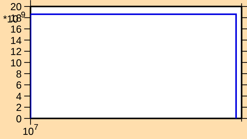
\sigma vs. E for ^{131}\text{Xe}(n,\text{nd})
