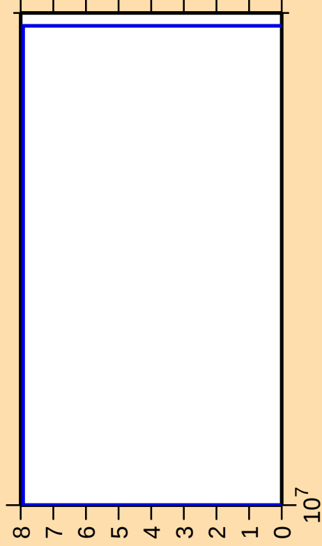
\Delta\sigma/\sigma vs. E for ^{131}\text{Xe}(n,nt)
