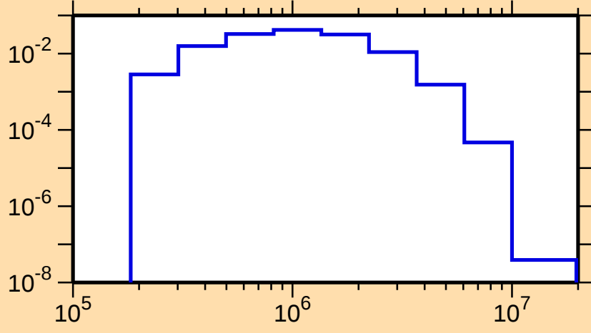
\sigma vs. E for ^{131}\text{Xe}(n,n_4)
