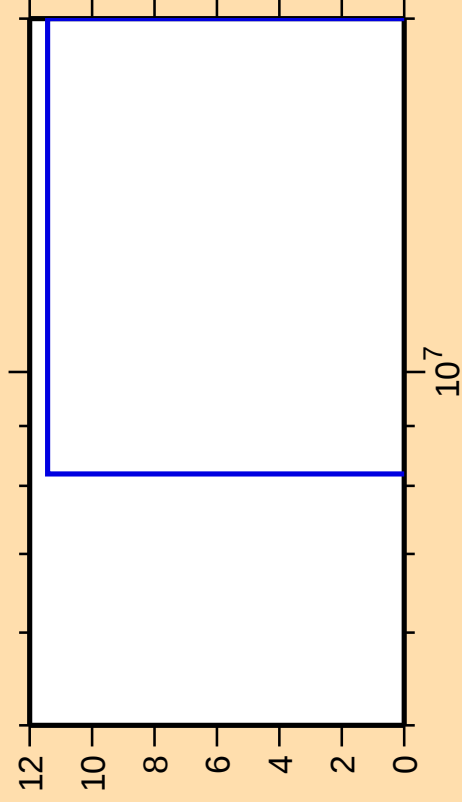
\Delta\sigma/\sigma vs. E for ^{131}\text{Xe}(n,nt)
