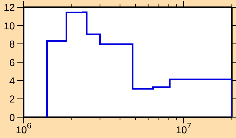
\Delta\sigma/\sigma vs. E for ^{131}\text{Xe}(n,\text{tot.})
