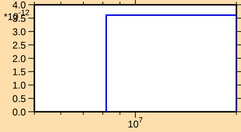
\sigma vs. E for ^{131}\text{Xe}(n,\text{He}3)
