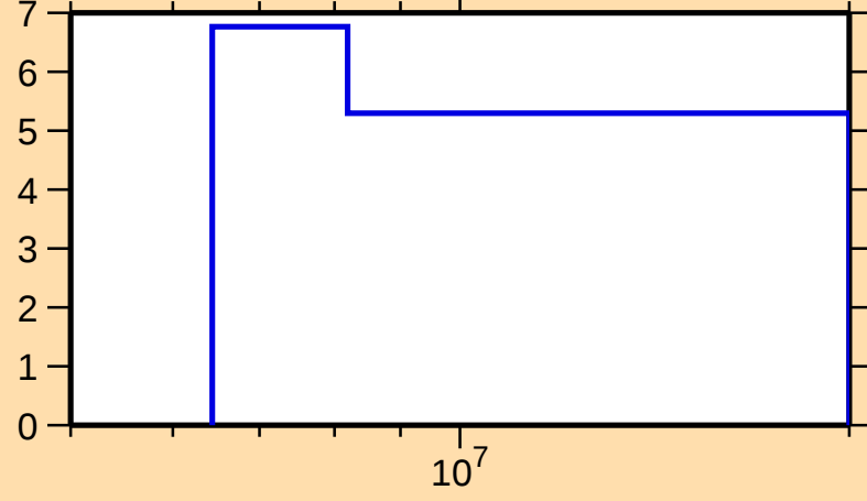
\Delta\sigma/\sigma vs. E for ^{131}\text{Xe}(n,\text{nonel.})
