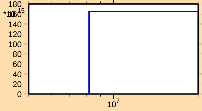
\sigma vs. E for ^{131}\text{Xe}(n,p\alpha)
