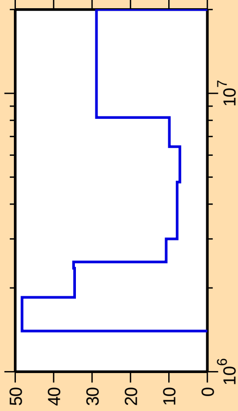
\Delta\sigma/\sigma vs. E for ^{131}\text{Xe}(n,\text{ncont.})
