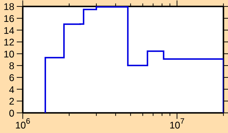
\Delta\sigma/\sigma vs. E for ^{131}\text{Xe}(n,\text{el.})
