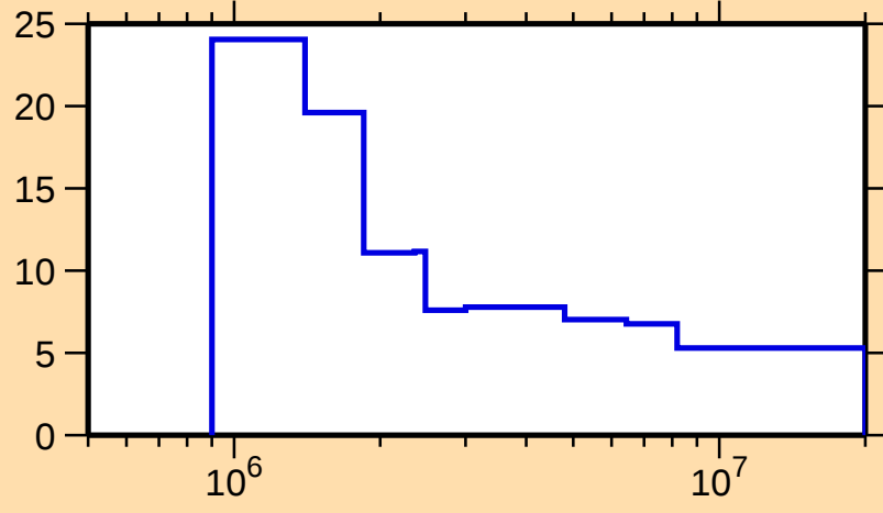
\Delta\sigma/\sigma vs. E for ^{131}\text{Xe}(n,\text{nonel.})
