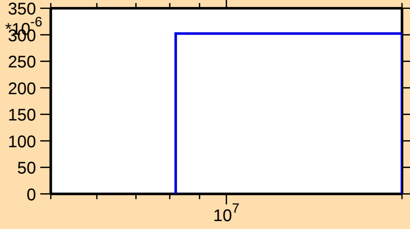
\sigma vs. E for ^{131}\text{Xe}(n,np)
