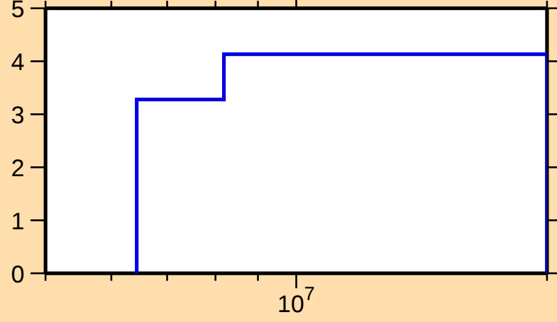
\Delta\sigma/\sigma vs. E for ^{131}\text{Xe}(n,\text{tot.})
