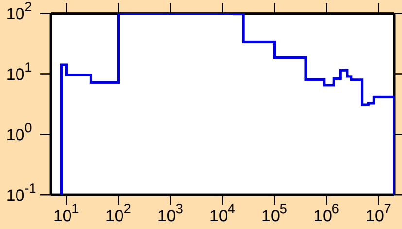
\Delta\sigma/\sigma vs. E for ^{131}\text{Xe}(n,\text{tot.})
