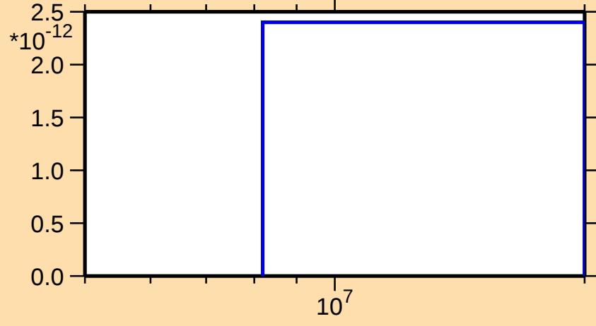
\sigma vs. E for ^{131}\text{Xe}(n,nt)
