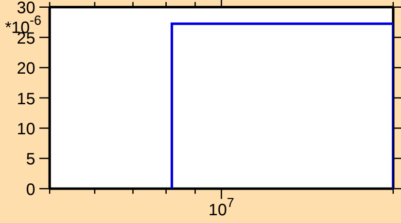
\sigma vs. E for ^{131}\text{Xe}(n,t)
