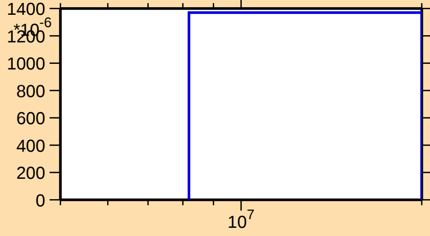
\sigma vs. E for ^{131}\text{Xe}(n,3n)
