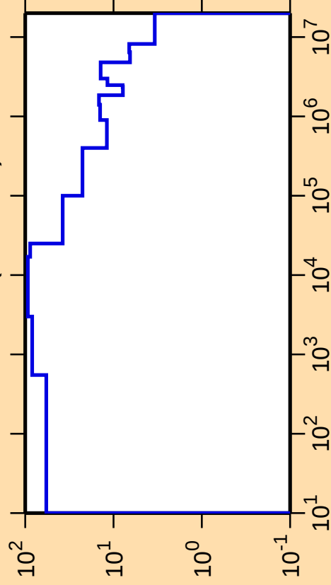
\Delta\sigma/\sigma vs. E for ^{135}\text{Xe}(n,\text{nonel.})
