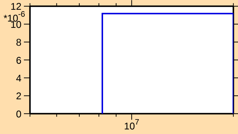
\sigma vs. E for ^{135}\text{Xe}(n,n\alpha)
