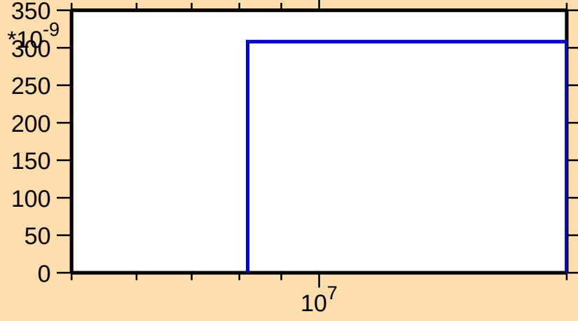
\sigma vs. E for ^{141}\text{Xe}(n,nt)
