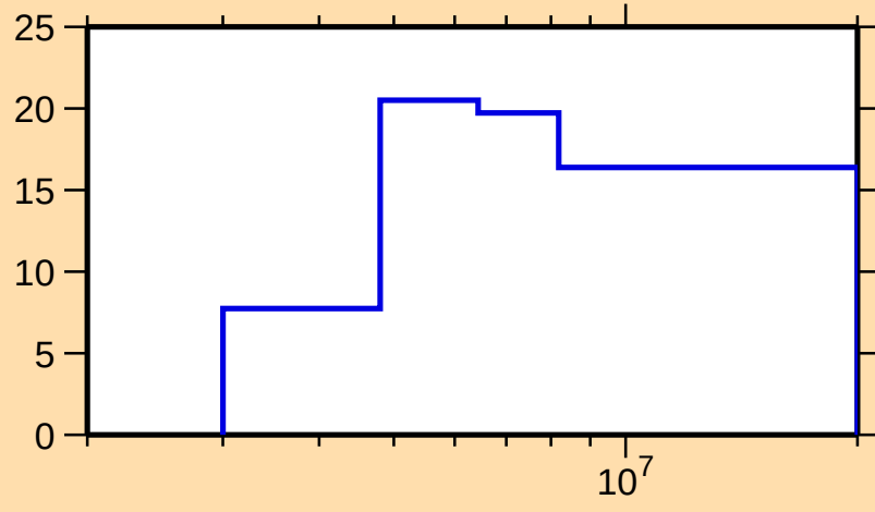
\Delta\sigma/\sigma vs. E for ^{141}\text{Xe}(n,\text{tot.})
