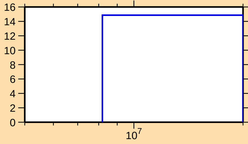
\Delta\sigma/\sigma vs. E for ^{141}\text{Xe}(n,\text{nonel.})
