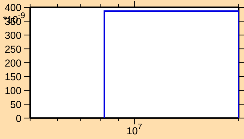
\sigma vs. E for ^{141}\text{Xe}(n,2n\alpha)
