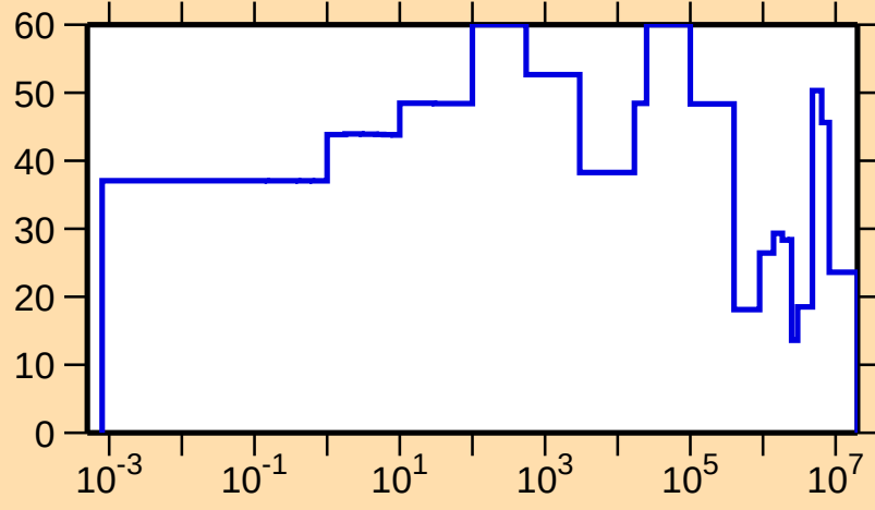
\Delta\sigma/\sigma vs. E for ^{141}\text{Xe}(n,\text{el.})
