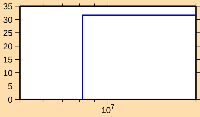
\Delta\sigma/\sigma vs. E for ^{141}\text{Xe}(n,n\text{cont.})
