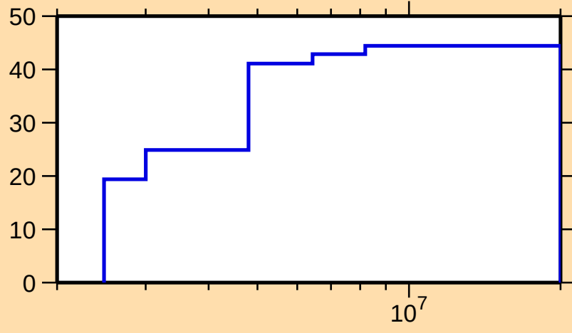
\Delta\sigma/\sigma vs. E for ^{141}\text{Xe}(n,\text{inel.})
