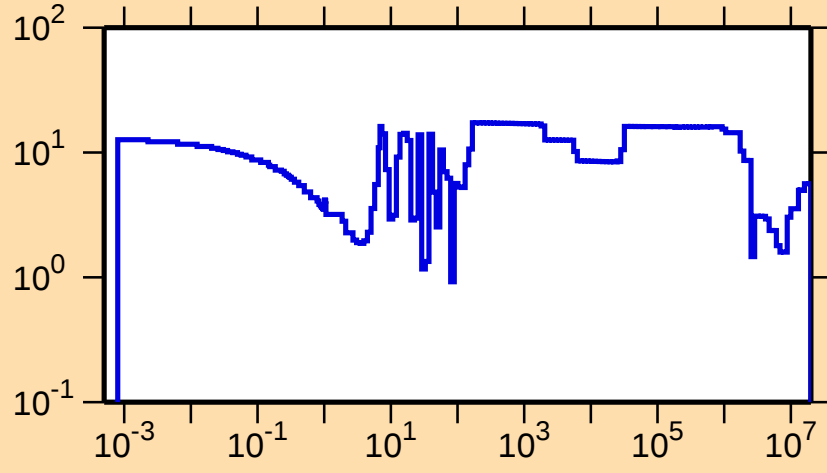
\Delta\sigma/\sigma vs. E for ^{83}\text{Y}(\text{n,tot.})
