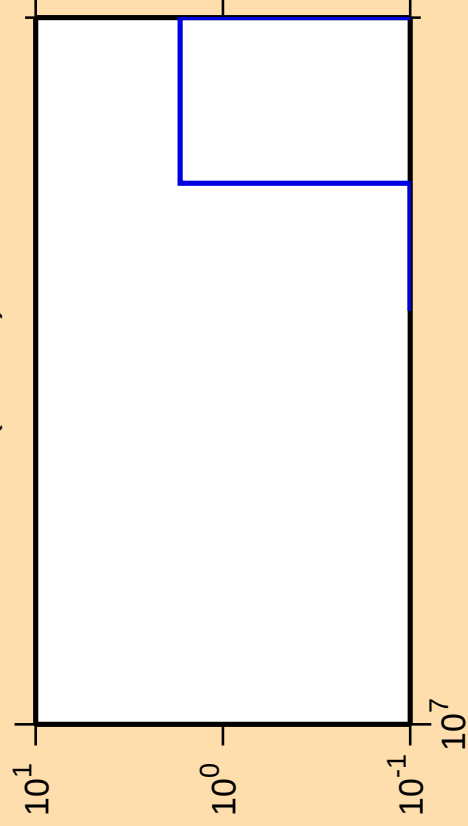
\Delta\sigma/\sigma vs. E for ^{83}\text{Y} (mt 34)
