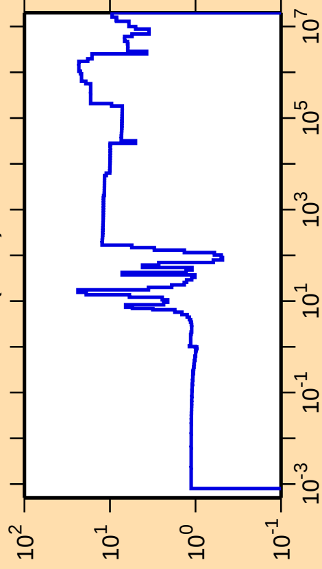
\Delta\sigma/\sigma vs. E for ^{83}\text{Y}(\text{n,el.})
