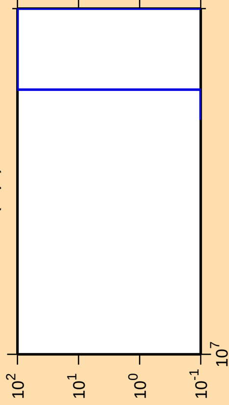
\Delta\sigma/\sigma vs. E for ^{83}\text{Y}(\text{n},\text{pt})
