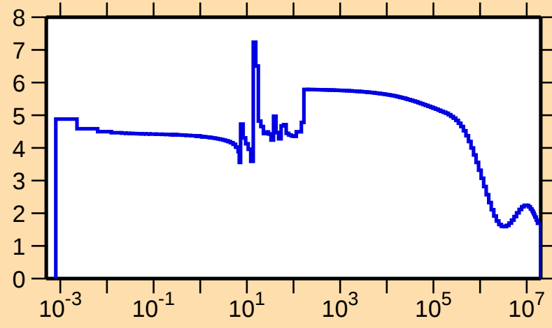
\sigma vs. E for ^{83}\text{Y}(n,\text{el.})
