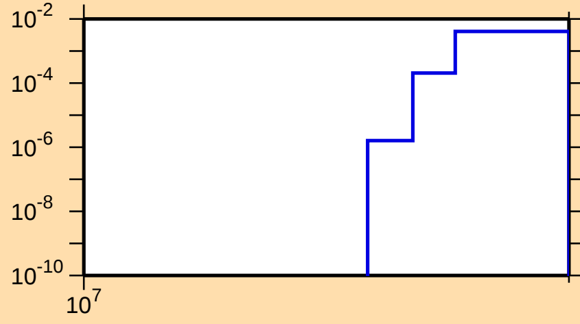
\sigma vs. E for ^{86}\text{Y}(n,2np)
