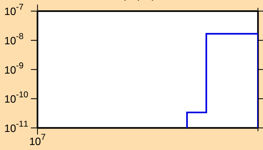
\sigma vs. E for ^{86}\text{Y}(n,\text{pd})
