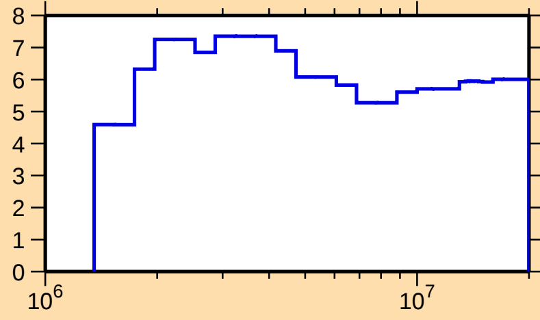
\Delta\sigma/\sigma vs. E for ^{86}\text{Y}(n,n\text{onel.})
