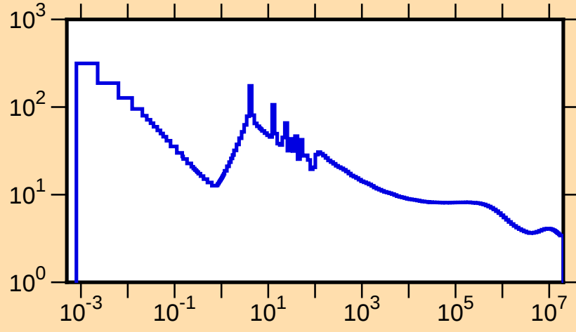
\sigma vs. E for ^{86}\text{Y}(n,\text{tot.})
